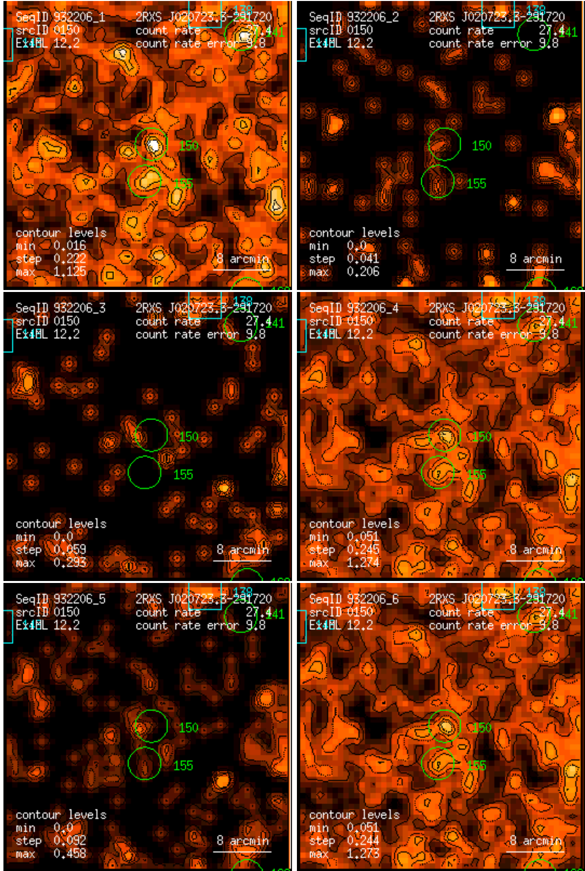
Figure 150: RASS 932206: detection 0150: band rate images, Gaussian filter: (1) PSPC channels 11 – 41, (2) 52 – 90, (3) 91 – 201, (4) 11 – 235, (5) 52 – 201, (6) 11 – 201. Broad band rates in counts/ks. Band rate contour levels in counts/ks/arcmin 2 .
