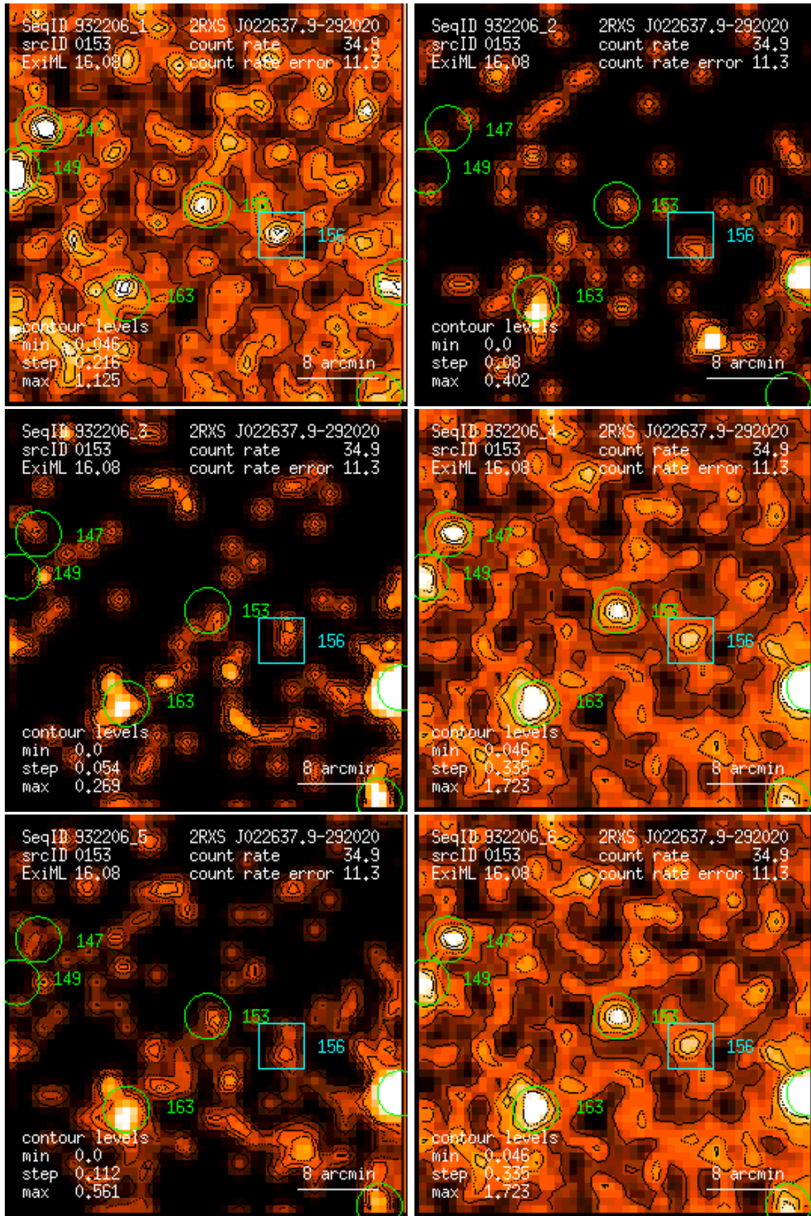
Figure 153: RASS 932206: detection 0153: band rate images, Gaussian filter: (1) PSPC channels 11 – 41, (2) 52 – 90, (3) 91 – 201, (4) 11 – 235, (5) 52 – 201, (6) 11 – 201. Broad band rates in counts/ks. Band rate contour levels in counts/ks/arcmin 2 .
