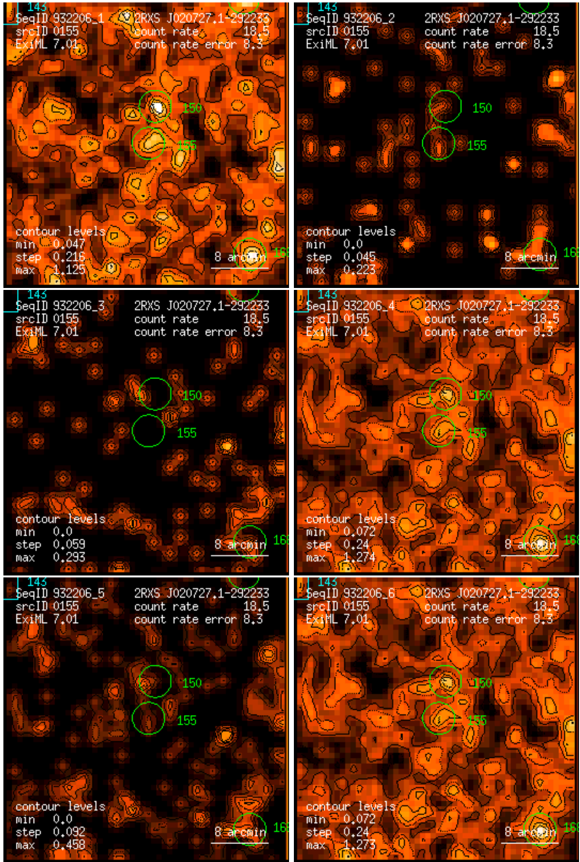
Figure 155: RASS 932206: detection 0155: band rate images, Gaussian filter: (1) PSPC channels 11 – 41, (2) 52 – 90, (3) 91 – 201, (4) 11 – 235, (5) 52 – 201, (6) 11 – 201. Broad band rates in counts/ks. Band rate contour levels in counts/ks/arcmin 2 .
