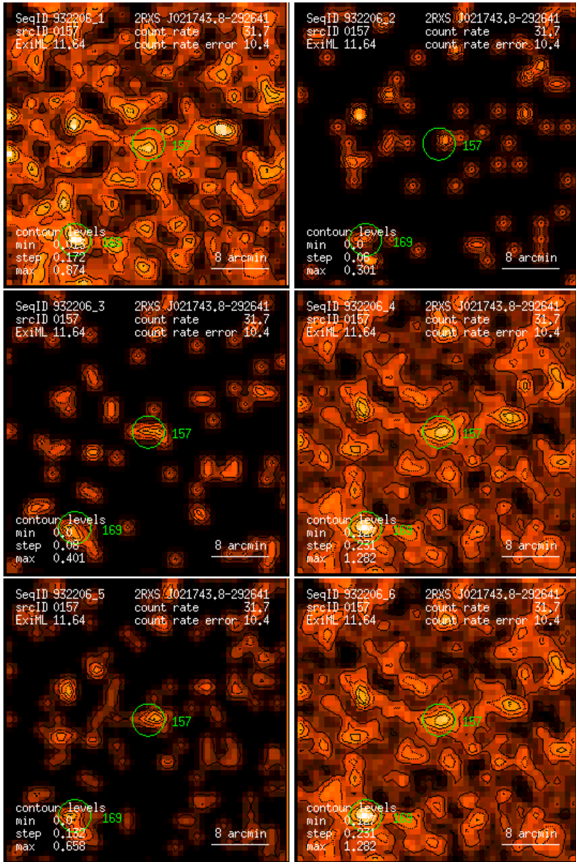
Figure 157: RASS 932206: detection 0157: band rate images, Gaussian filter: (1) PSPC channels 11 – 41, (2) 52 – 90, (3) 91 – 201, (4) 11 – 235, (5) 52 – 201, (6) 11 – 201. Broad band rates in counts/ks. Band rate contour levels in counts/ks/arcmin 2 .
