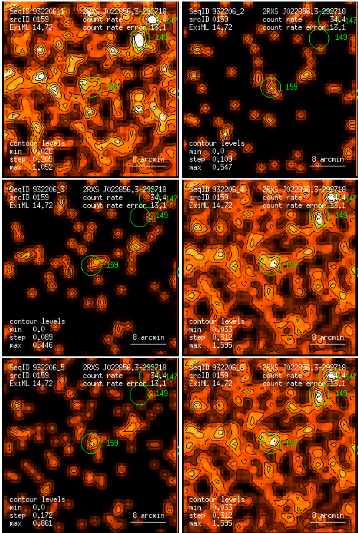
Figure 159: RASS 932206: detection 0159: band rate images, Gaussian filter: (1) PSPC channels 11 – 41, (2) 52 – 90, (3) 91 – 201, (4) 11 – 235, (5) 52 – 201, (6) 11 – 201. Broad band rates in counts/ks. Band rate contour levels in counts/ks/arcmin 2 .
