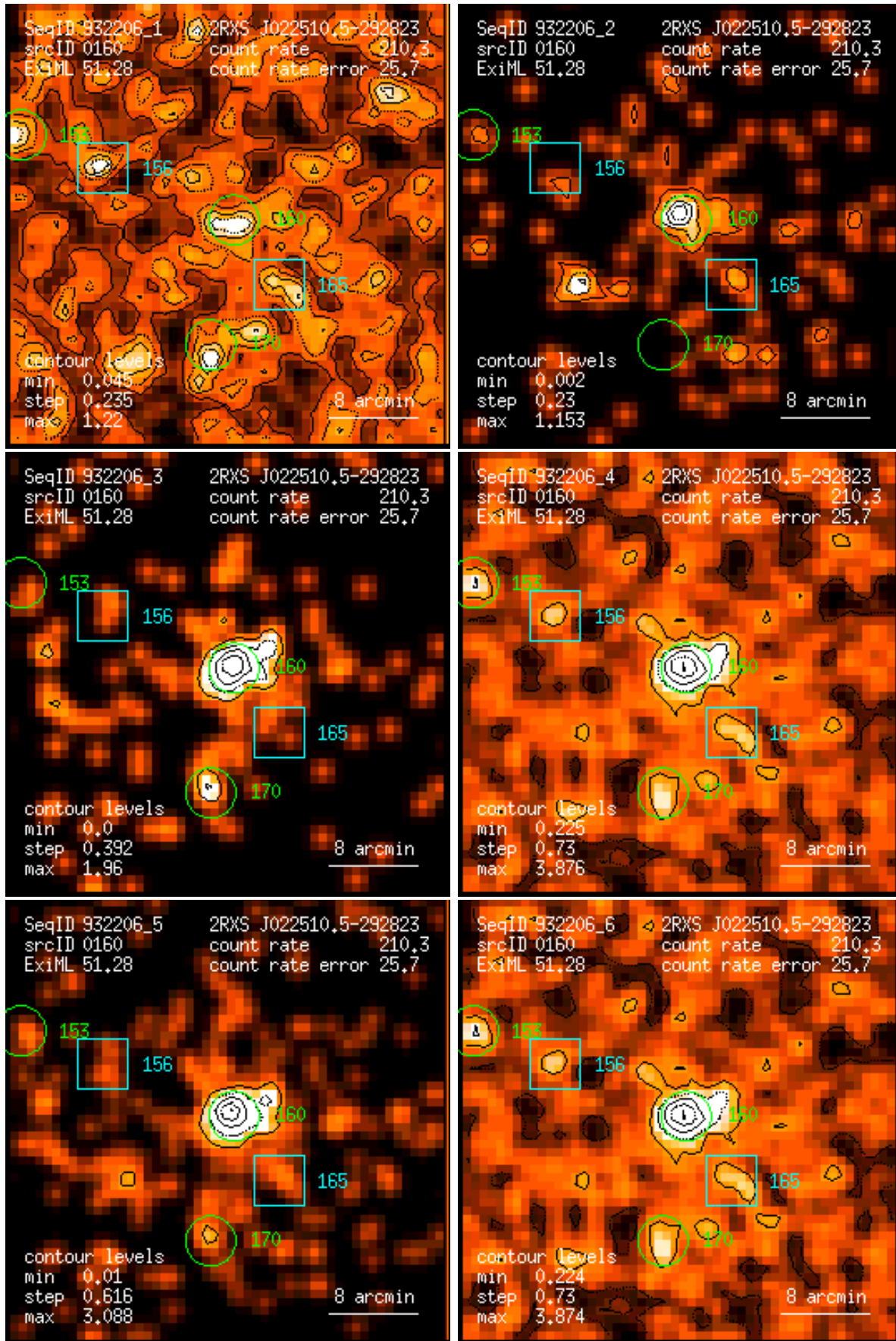
Figure 160: RASS 932206: detection 0160: band rate images, Gaussian filter: (1) PSPC channels 11 – 41, (2) 52 – 90, (3) 91 – 201, (4) 11 – 235, (5) 52 – 201, (6) 11 – 201. Broad band rates in counts/ks. Band rate contour levels in counts/ks/arcmin 2 .
