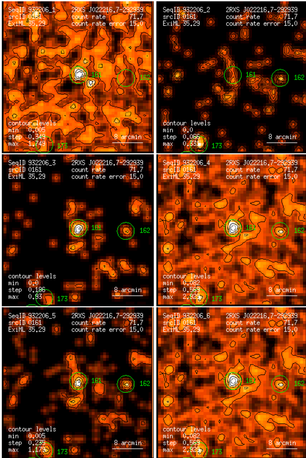
Figure 161: RASS 932206: detection 0161: band rate images, Gaussian filter: (1) PSPC channels 11 – 41, (2) 52 – 90, (3) 91 – 201, (4) 11 – 235, (5) 52 – 201, (6) 11 – 201. Broad band rates in counts/ks. Band rate contour levels in counts/ks/arcmin 2 .
