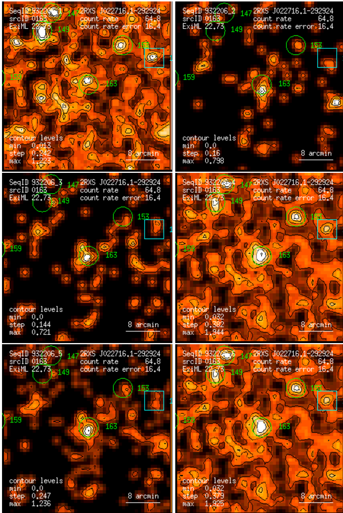
Figure 163: RASS 932206: detection 0163: band rate images, Gaussian filter: (1) PSPC channels 11 – 41, (2) 52 – 90, (3) 91 – 201, (4) 11 – 235, (5) 52 – 201, (6) 11 – 201. Broad band rates in counts/ks. Band rate contour levels in counts/ks/arcmin 2 .
