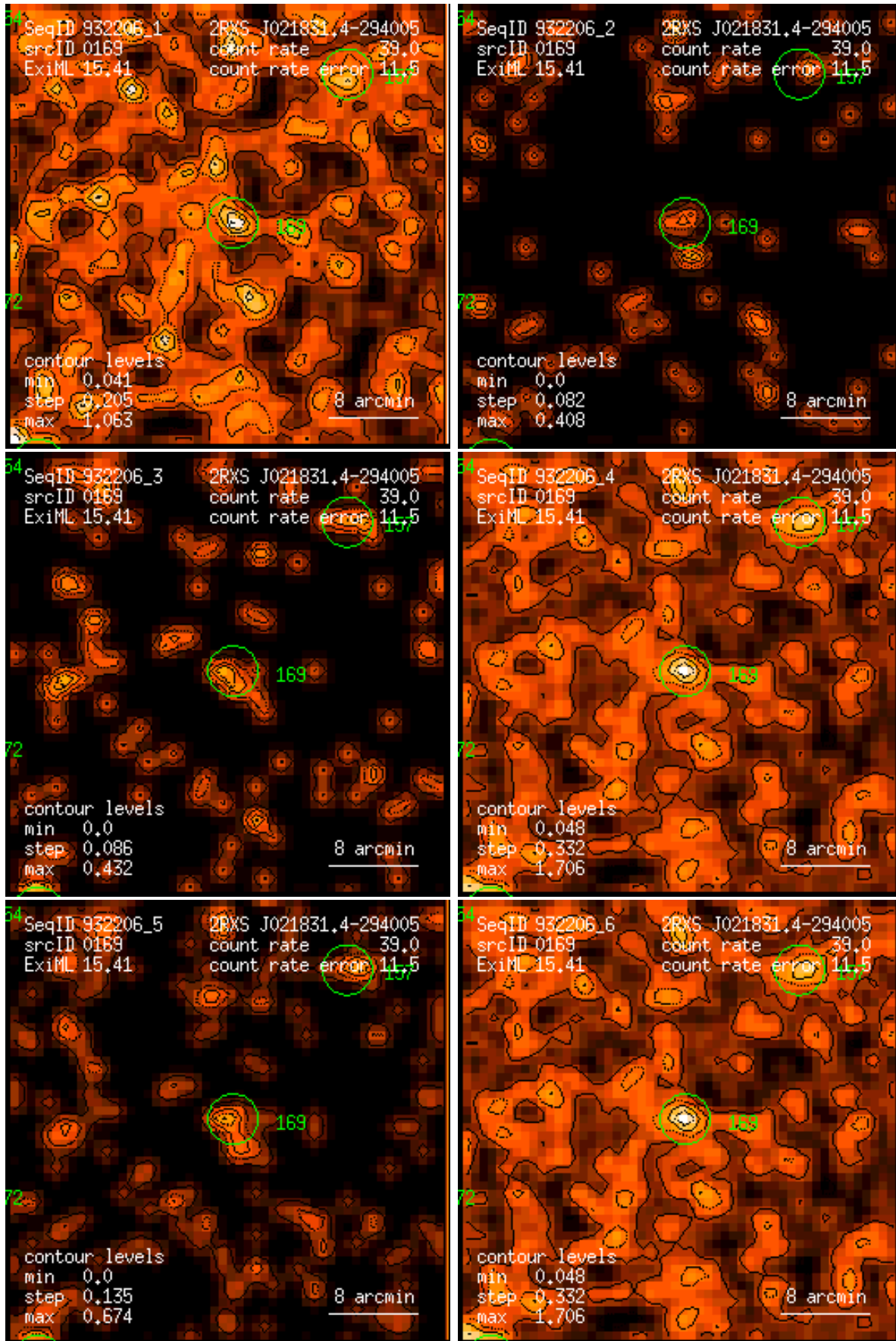
Figure 169: RASS 932206: detection 0169: band rate images, Gaussian filter: (1) PSPC channels 11 – 41, (2) 52 – 90, (3) 91 – 201, (4) 11 – 235, (5) 52 – 201, (6) 11 – 201. Broad band rates in counts/ks. Band rate contour levels in counts/ks/arcmin 2 .
