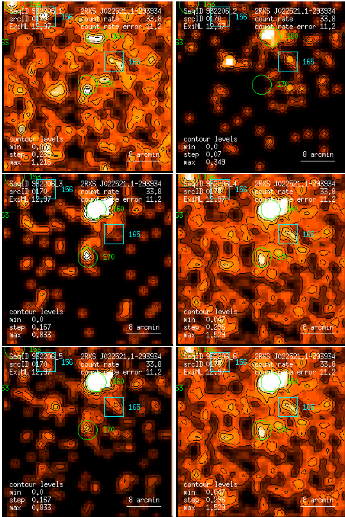
Figure 170: RASS 932206: detection 0170: band rate images, Gaussian filter: (1) PSPC channels 11 – 41, (2) 52 – 90, (3) 91 – 201, (4) 11 – 235, (5) 52 – 201, (6) 11 – 201. Broad band rates in counts/ks. Band rate contour levels in counts/ks/arcmin 2 .
