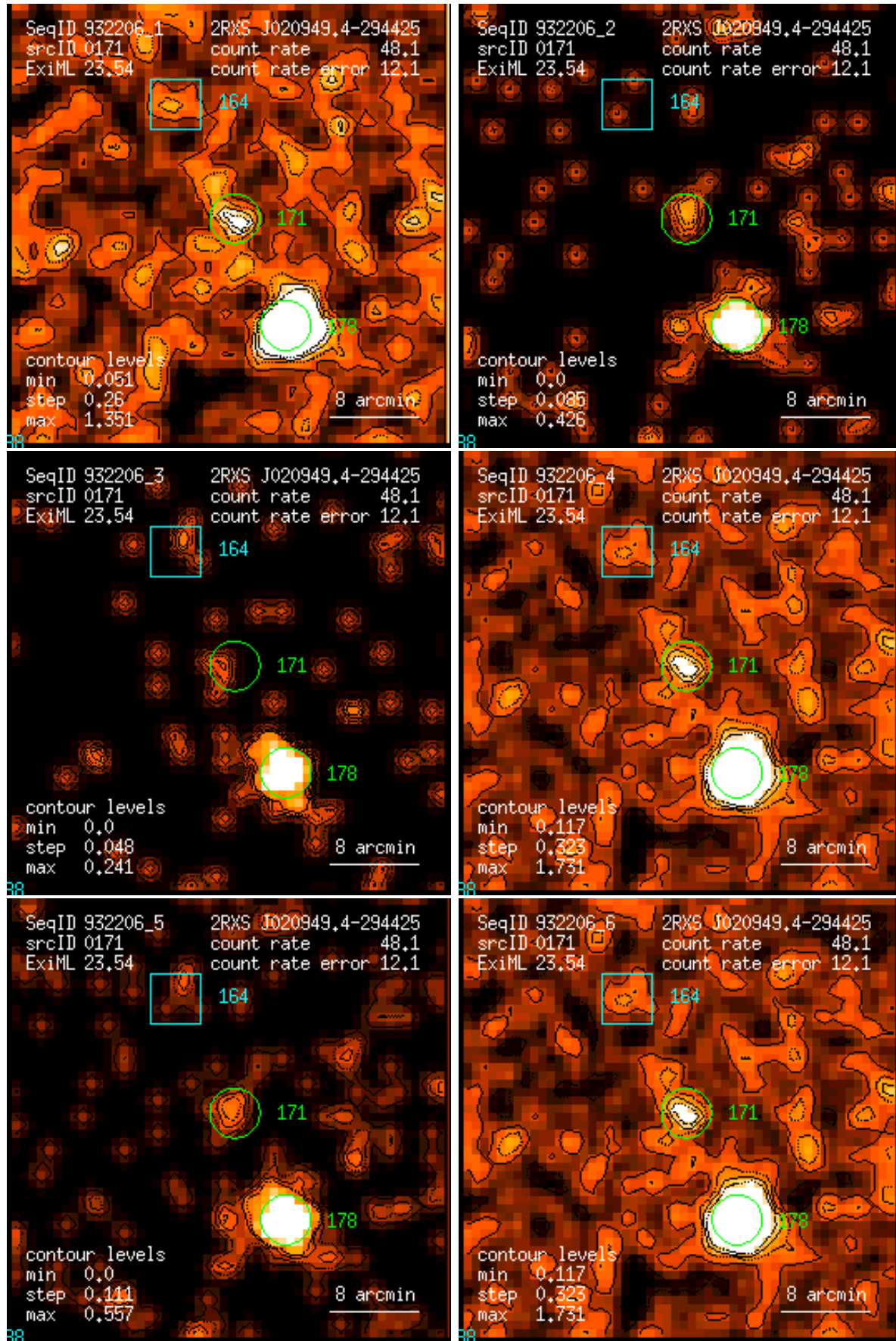
Figure 171: RASS 932206: detection 0171: band rate images, Gaussian filter: (1) PSPC channels 11 – 41, (2) 52 – 90, (3) 91 – 201, (4) 11 – 235, (5) 52 – 201, (6) 11 – 201. Broad band rates in counts/ks. Band rate contour levels in counts/ks/arcmin 2 .
