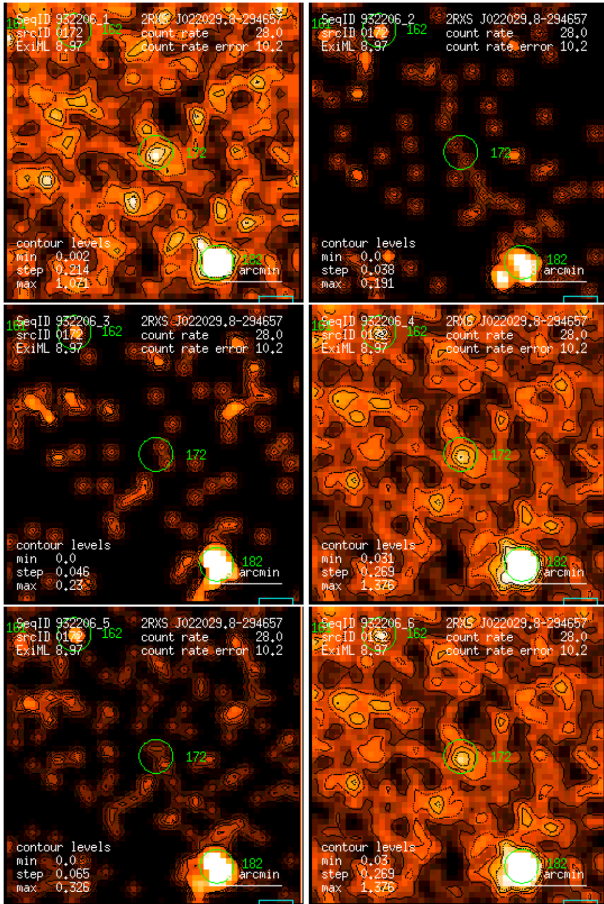
Figure 172: RASS 932206: detection 0172: band rate images, Gaussian filter: (1) PSPC channels 11 – 41, (2) 52 – 90, (3) 91 – 201, (4) 11 – 235, (5) 52 – 201, (6) 11 – 201. Broad band rates in counts/ks. Band rate contour levels in counts/ks/arcmin 2 .
