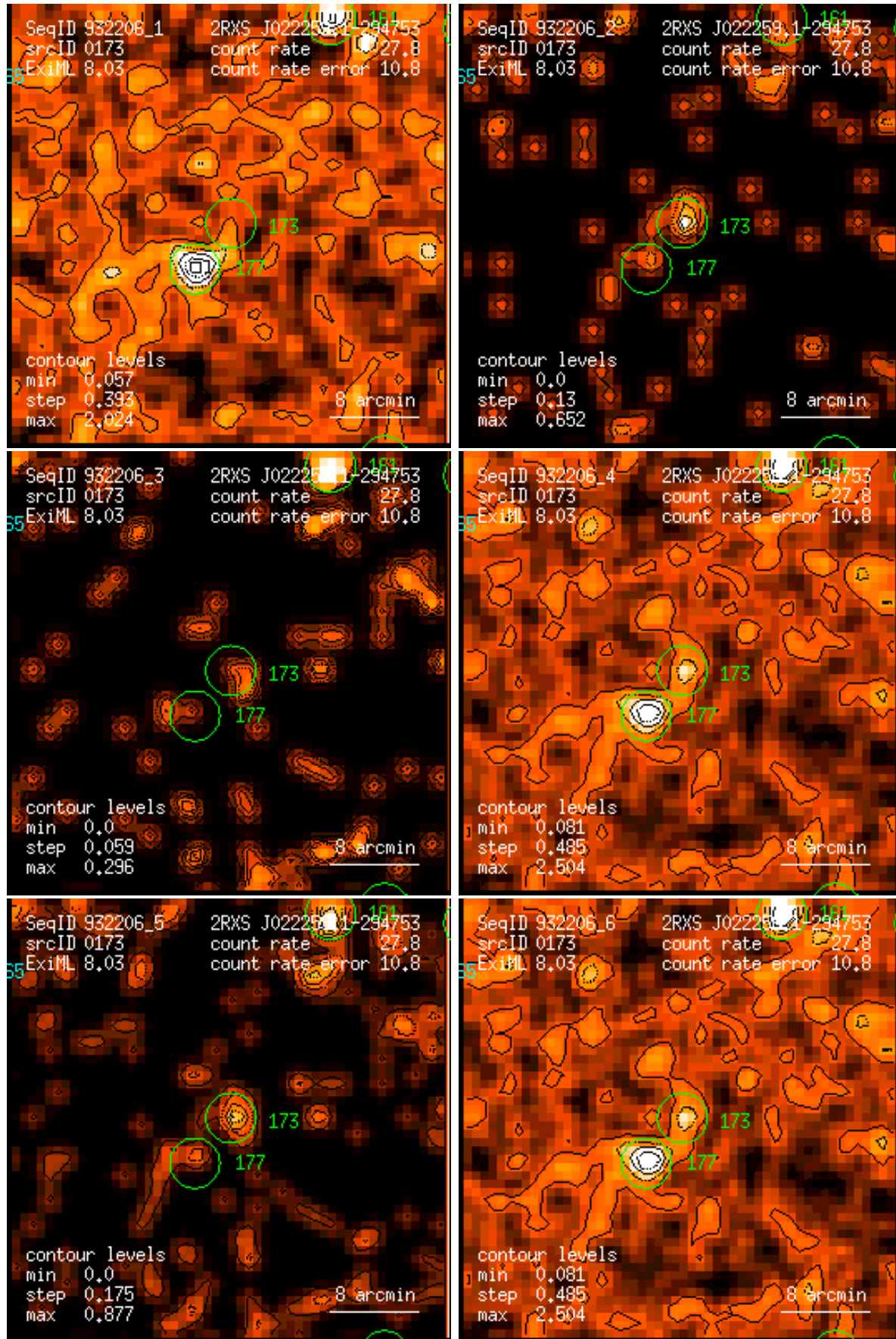
Figure 173: RASS 932206: detection 0173: band rate images, Gaussian filter: (1) PSPC channels 11 – 41, (2) 52 – 90, (3) 91 – 201, (4) 11 – 235, (5) 52 – 201, (6) 11 – 201. Broad band rates in counts/ks. Band rate contour levels in counts/ks/arcmin 2 .
