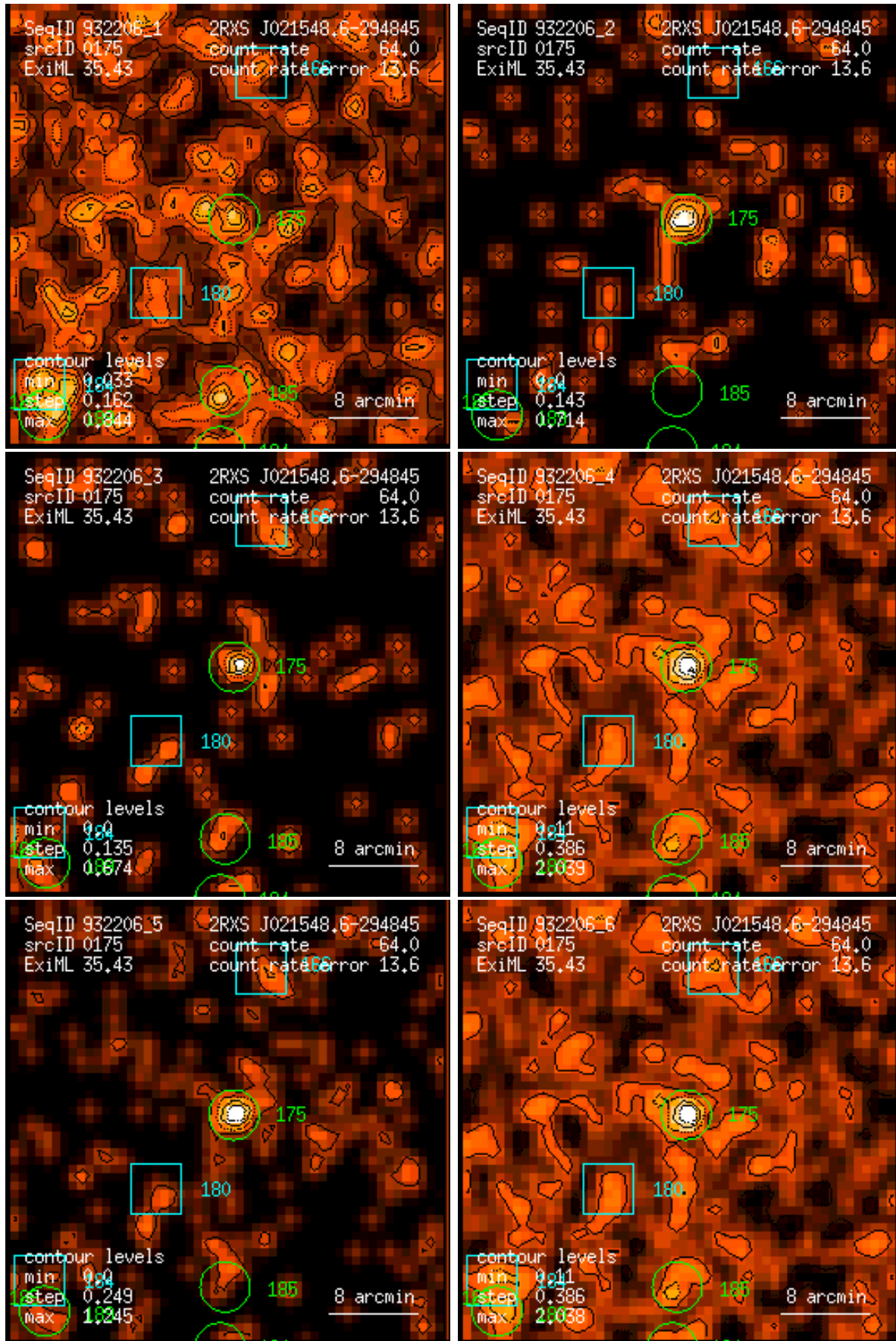
Figure 175: RASS 932206: detection 0175: band rate images, Gaussian filter: (1) PSPC channels 11 – 41, (2) 52 – 90, (3) 91 – 201, (4) 11 – 235, (5) 52 – 201, (6) 11 – 201. Broad band rates in counts/ks. Band rate contour levels in counts/ks/arcmin 2 .
