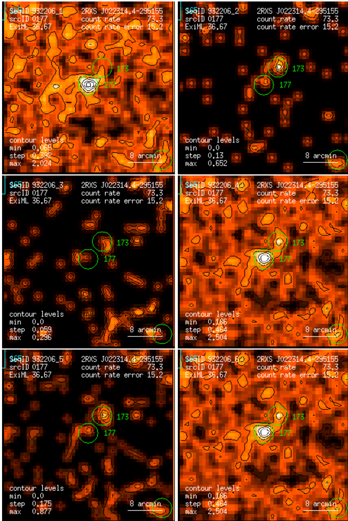
Figure 177: RASS 932206: detection 0177: band rate images, Gaussian filter: (1) PSPC channels 11 – 41, (2) 52 – 90, (3) 91 – 201, (4) 11 – 235, (5) 52 – 201, (6) 11 – 201. Broad band rates in counts/ks. Band rate contour levels in counts/ks/arcmin 2 .
