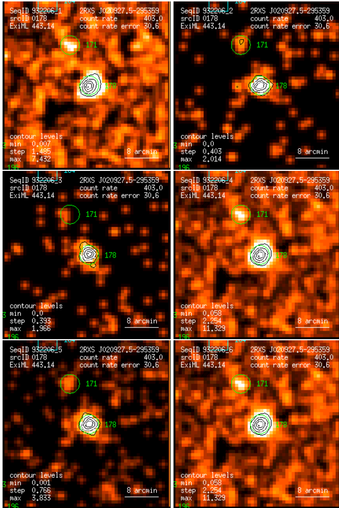
Figure 178: RASS 932206: detection 0178: band rate images, Gaussian filter: (1) PSPC channels 11 – 41, (2) 52 – 90, (3) 91 – 201, (4) 11 – 235, (5) 52 – 201, (6) 11 – 201. Broad band rates in counts/ks. Band rate contour levels in counts/ks/arcmin 2 .
