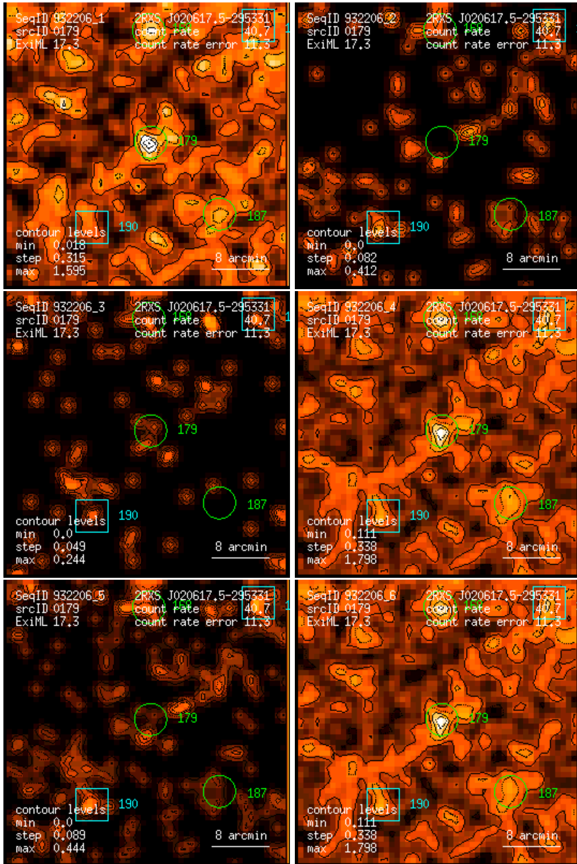
Figure 179: RASS 932206: detection 0179: band rate images, Gaussian filter: (1) PSPC channels 11 – 41, (2) 52 – 90, (3) 91 – 201, (4) 11 – 235, (5) 52 – 201, (6) 11 – 201. Broad band rates in counts/ks. Band rate contour levels in counts/ks/arcmin 2 .
