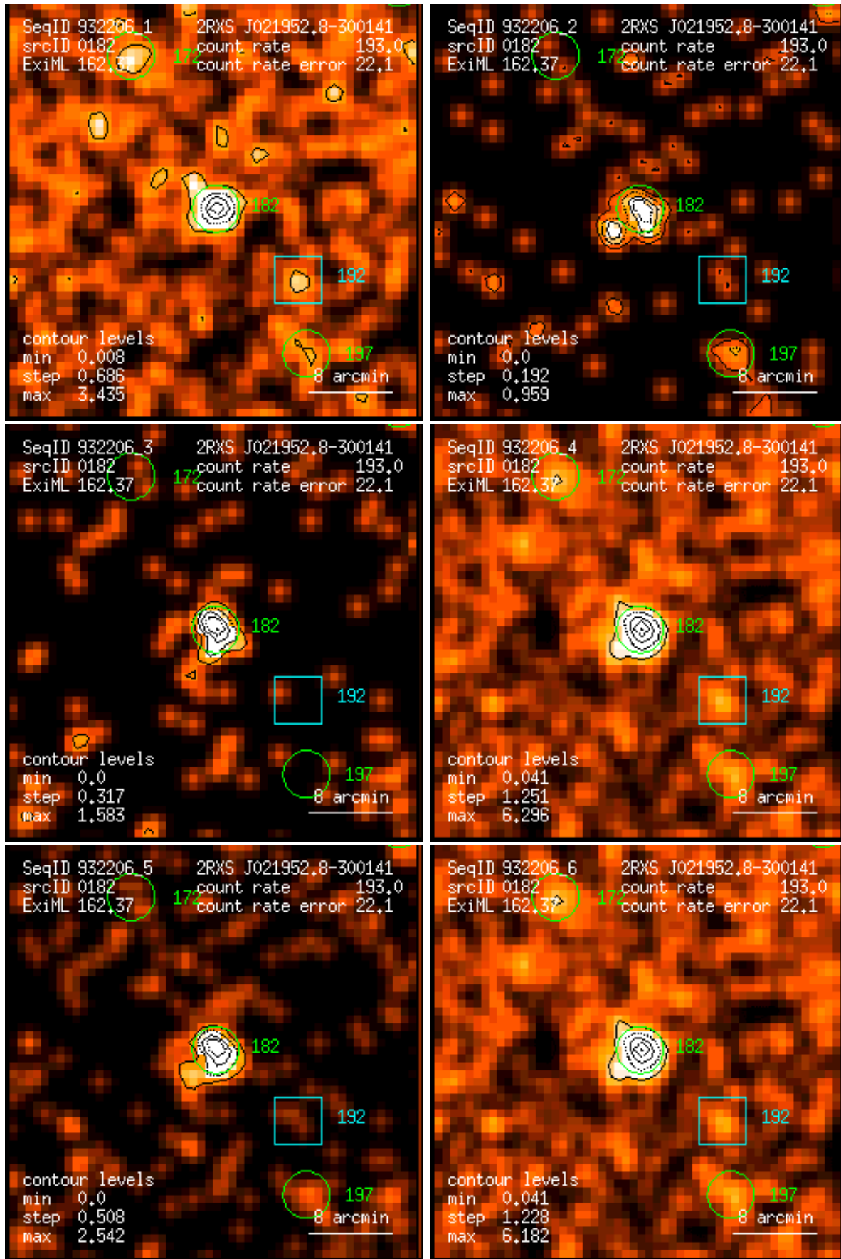
Figure 182: RASS 932206: detection 0182: band rate images, Gaussian filter: (1) PSPC channels 11 – 41, (2) 52 – 90, (3) 91 – 201, (4) 11 – 235, (5) 52 – 201, (6) 11 – 201. Broad band rates in counts/ks. Band rate contour levels in counts/ks/arcmin 2 .
