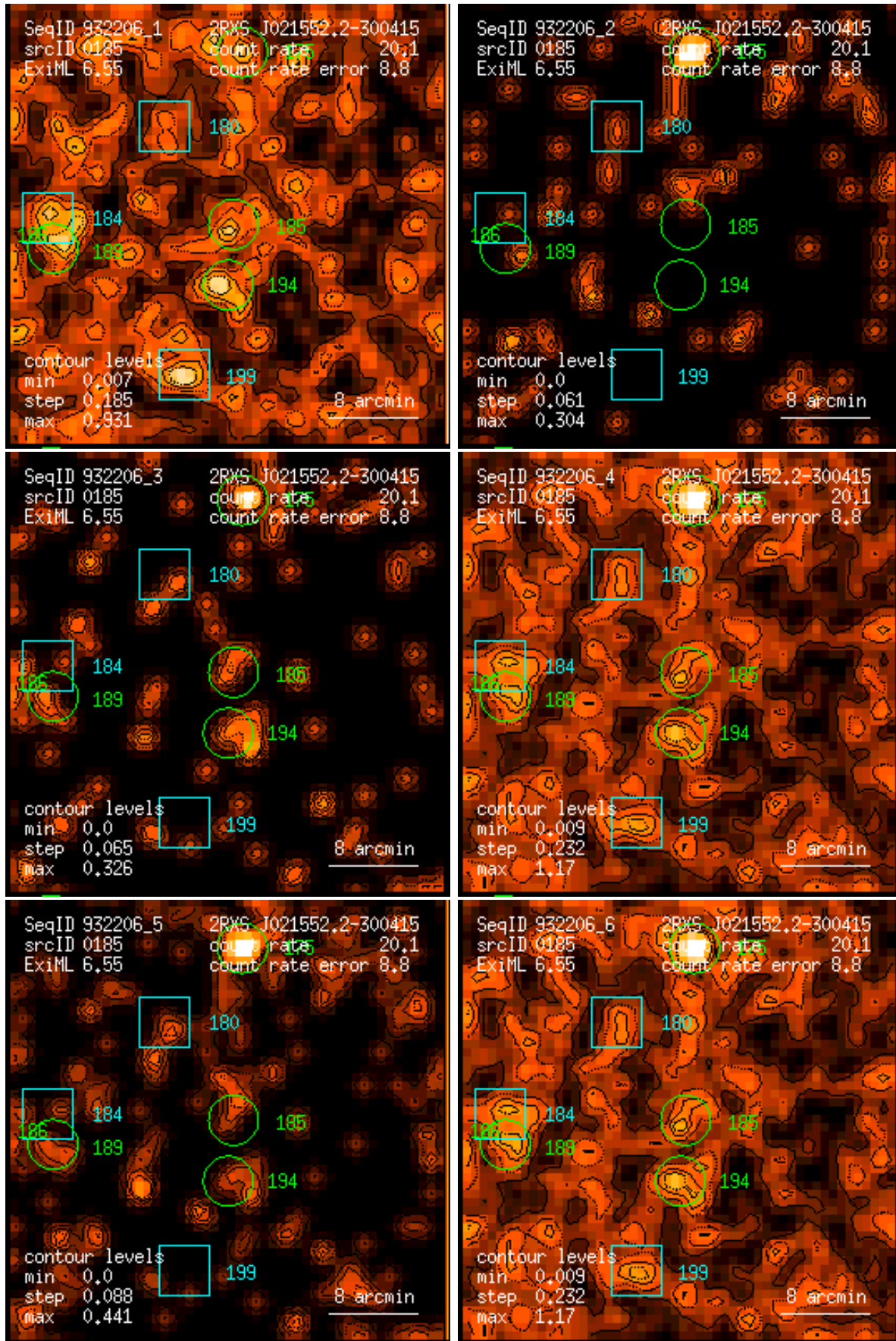
Figure 185: RASS 932206: detection 0185: band rate images, Gaussian filter: (1) PSPC channels 11 – 41, (2) 52 – 90, (3) 91 – 201, (4) 11 – 235, (5) 52 – 201, (6) 11 – 201. Broad band rates in counts/ks. Band rate contour levels in counts/ks/arcmin 2 .
