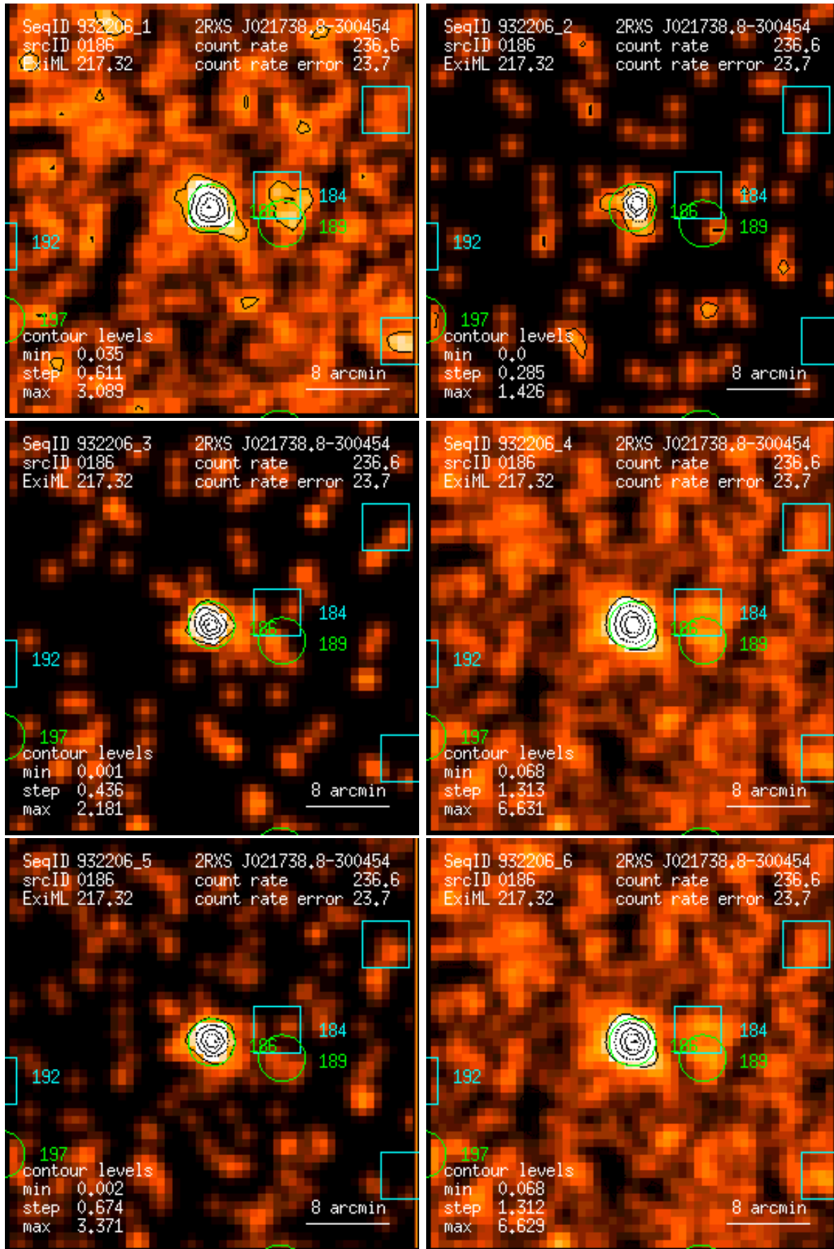
Figure 186: RASS 932206: detection 0186: band rate images, Gaussian filter: (1) PSPC channels 11 – 41, (2) 52 – 90, (3) 91 – 201, (4) 11 – 235, (5) 52 – 201, (6) 11 – 201. Broad band rates in counts/ks. Band rate contour levels in counts/ks/arcmin 2 .
