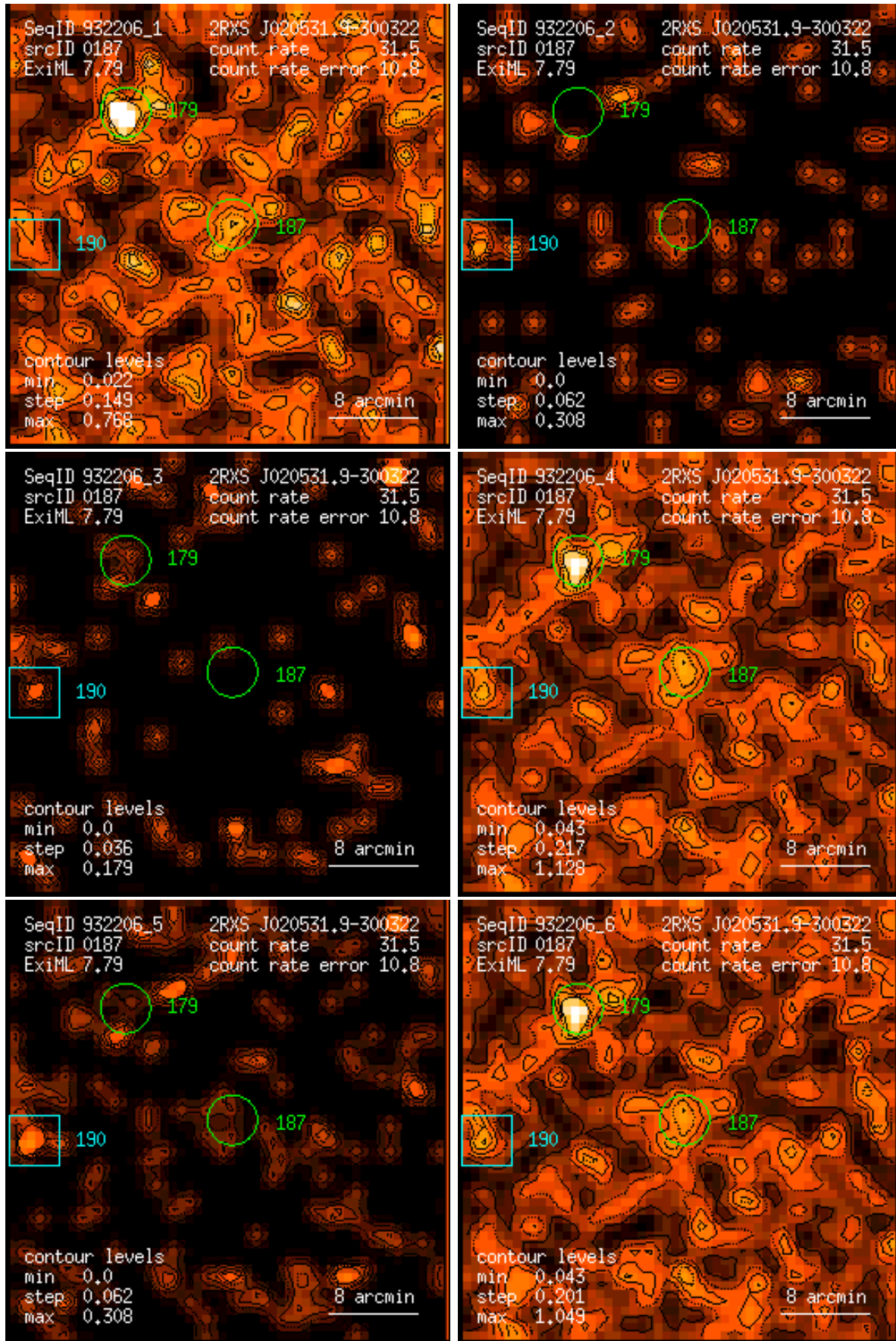
Figure 187: RASS 932206: detection 0187: band rate images, Gaussian filter: (1) PSPC channels 11 – 41, (2) 52 – 90, (3) 91 – 201, (4) 11 – 235, (5) 52 – 201, (6) 11 – 201. Broad band rates in counts/ks. Band rate contour levels in counts/ks/arcmin 2 .
