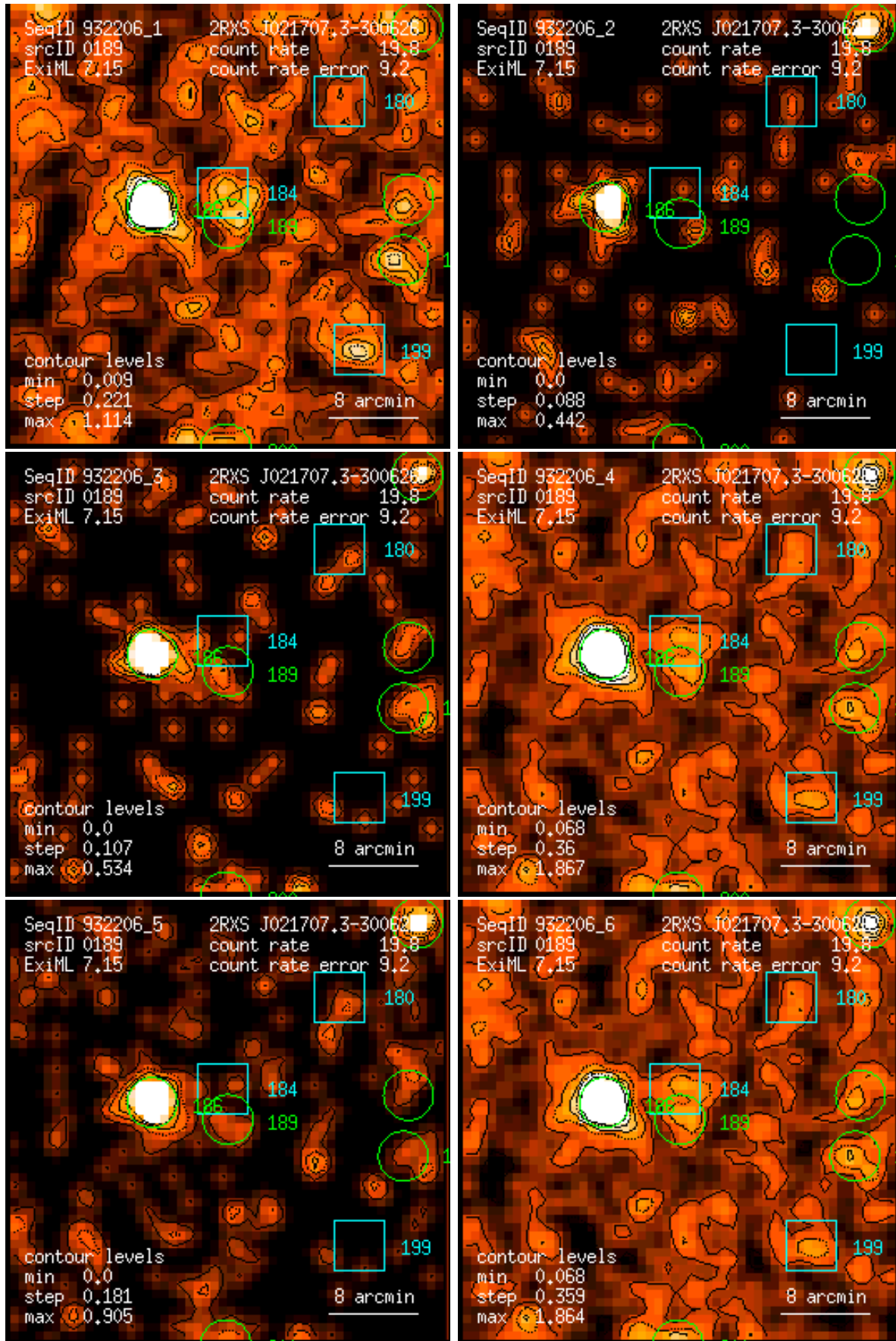
Figure 189: RASS 932206: detection 0189: band rate images, Gaussian filter: (1) PSPC channels 11 – 41, (2) 52 – 90, (3) 91 – 201, (4) 11 – 235, (5) 52 – 201, (6) 11 – 201. Broad band rates in counts/ks. Band rate contour levels in counts/ks/arcmin 2 .
