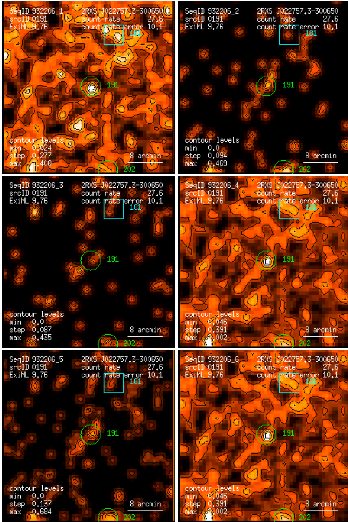
Figure 191: RASS 932206: detection 0191: band rate images, Gaussian filter: (1) PSPC channels 11 – 41, (2) 52 – 90, (3) 91 – 201, (4) 11 – 235, (5) 52 – 201, (6) 11 – 201. Broad band rates in counts/ks. Band rate contour levels in counts/ks/arcmin 2 .
