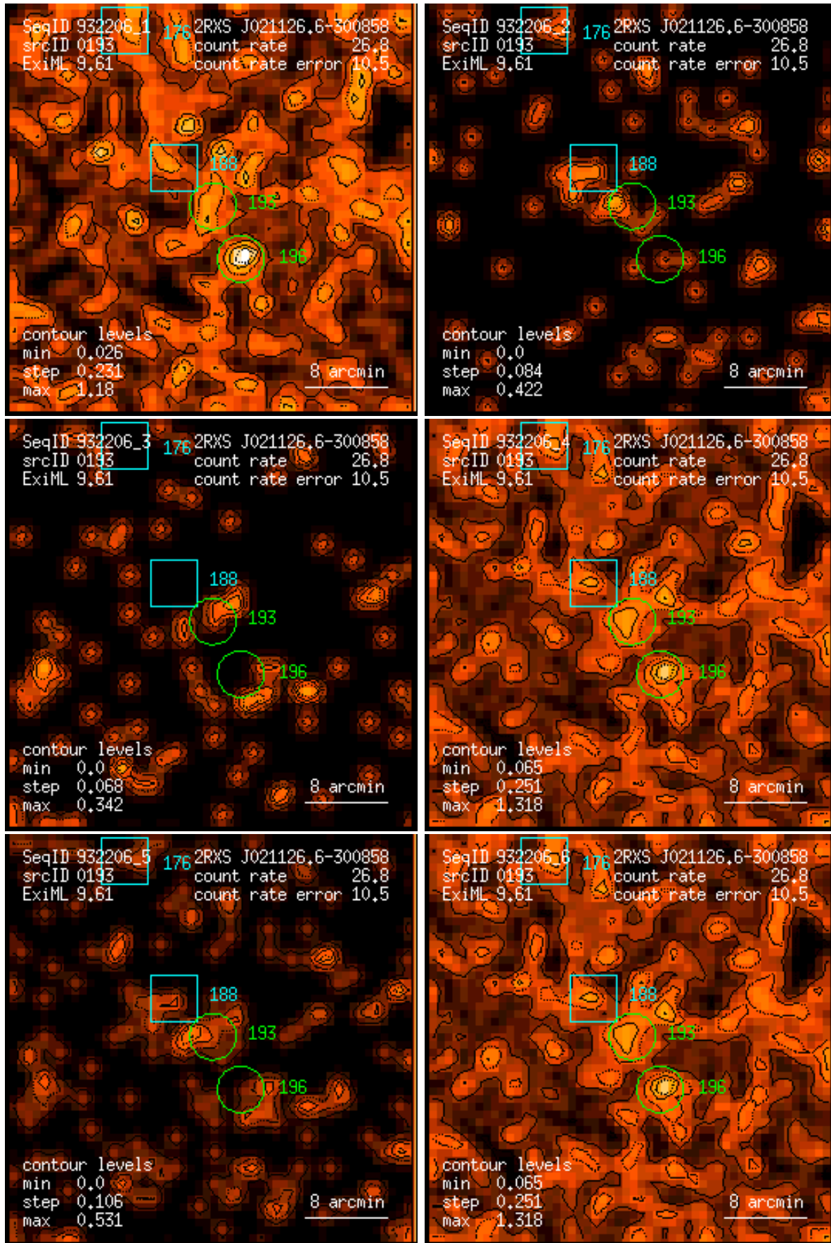
Figure 193: RASS 932206: detection 0193: band rate images, Gaussian filter: (1) PSPC channels 11 – 41, (2) 52 – 90, (3) 91 – 201, (4) 11 – 235, (5) 52 – 201, (6) 11 – 201. Broad band rates in counts/ks. Band rate contour levels in counts/ks/arcmin 2 .
