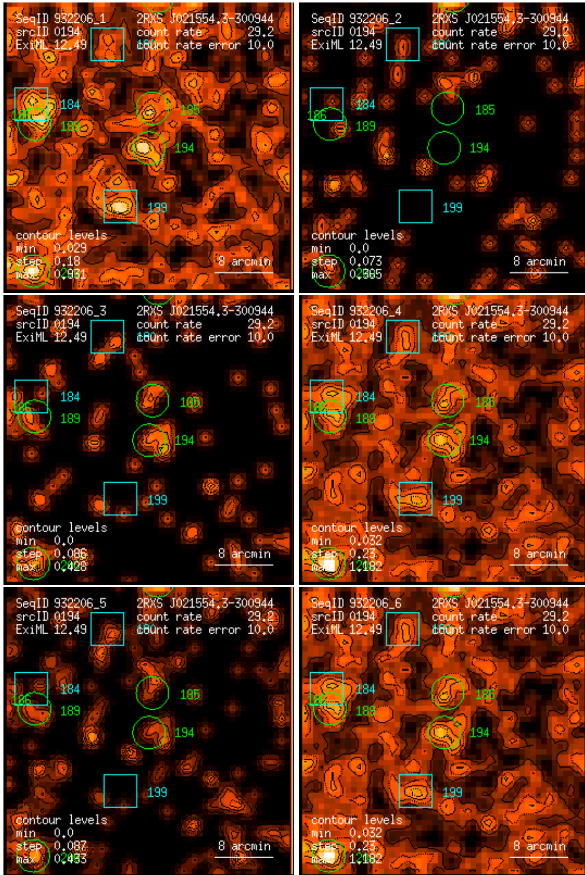
Figure 194: RASS 932206: detection 0194: band rate images, Gaussian filter: (1) PSPC channels 11 – 41, (2) 52 – 90, (3) 91 – 201, (4) 11 – 235, (5) 52 – 201, (6) 11 – 201. Broad band rates in counts/ks. Band rate contour levels in counts/ks/arcmin 2 .
