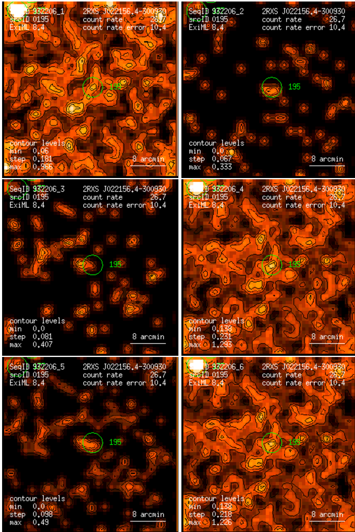
Figure 195: RASS 932206: detection 0195: band rate images, Gaussian filter: (1) PSPC channels 11 – 41, (2) 52 – 90, (3) 91 – 201, (4) 11 – 235, (5) 52 – 201, (6) 11 – 201. Broad band rates in counts/ks. Band rate contour levels in counts/ks/arcmin 2 .
