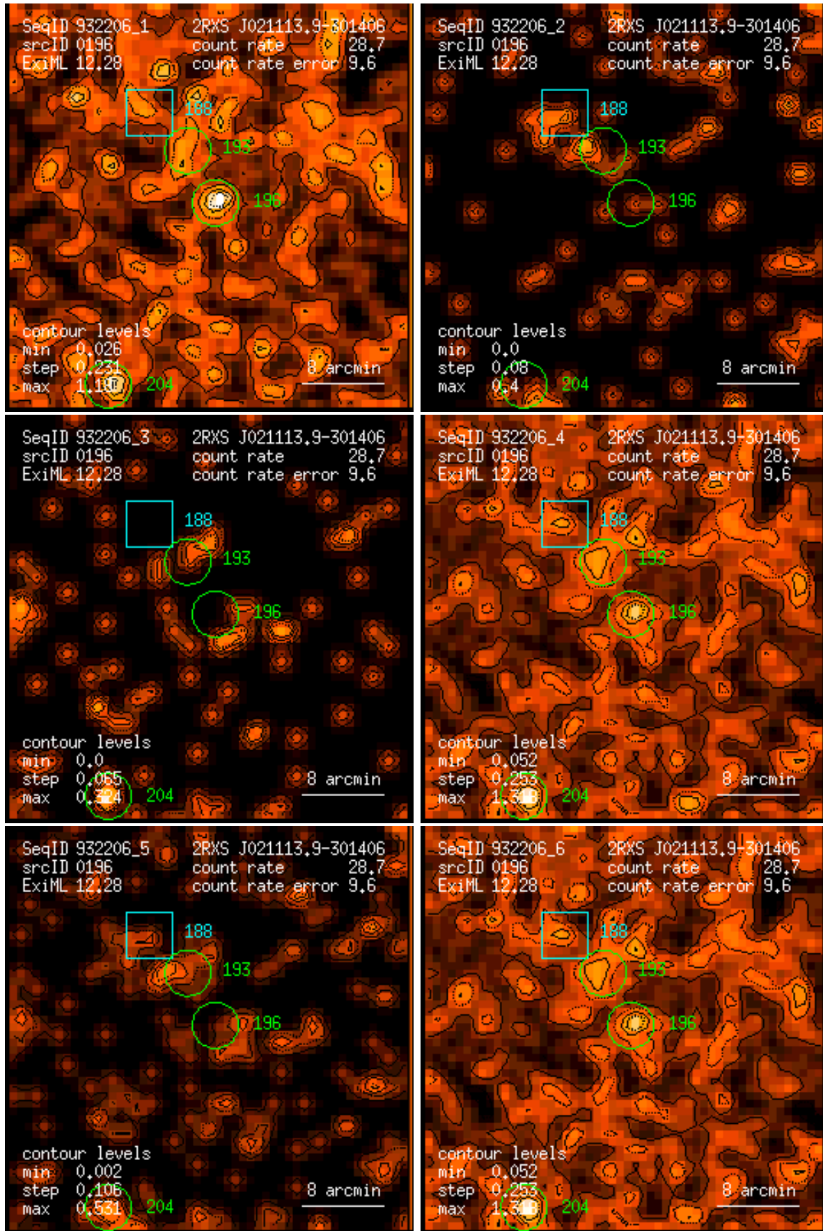
Figure 196: RASS 932206: detection 0196: band rate images, Gaussian filter: (1) PSPC channels 11 – 41, (2) 52 – 90, (3) 91 – 201, (4) 11 – 235, (5) 52 – 201, (6) 11 – 201. Broad band rates in counts/ks. Band rate contour levels in counts/ks/arcmin 2 .
