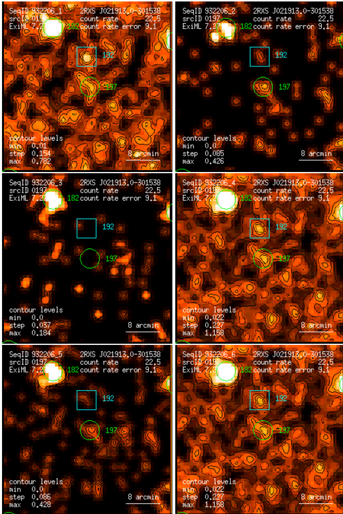
Figure 197: RASS 932206: detection 0197: band rate images, Gaussian filter: (1) PSPC channels 11 – 41, (2) 52 – 90, (3) 91 – 201, (4) 11 – 235, (5) 52 – 201, (6) 11 – 201. Broad band rates in counts/ks. Band rate contour levels in counts/ks/arcmin 2 .
