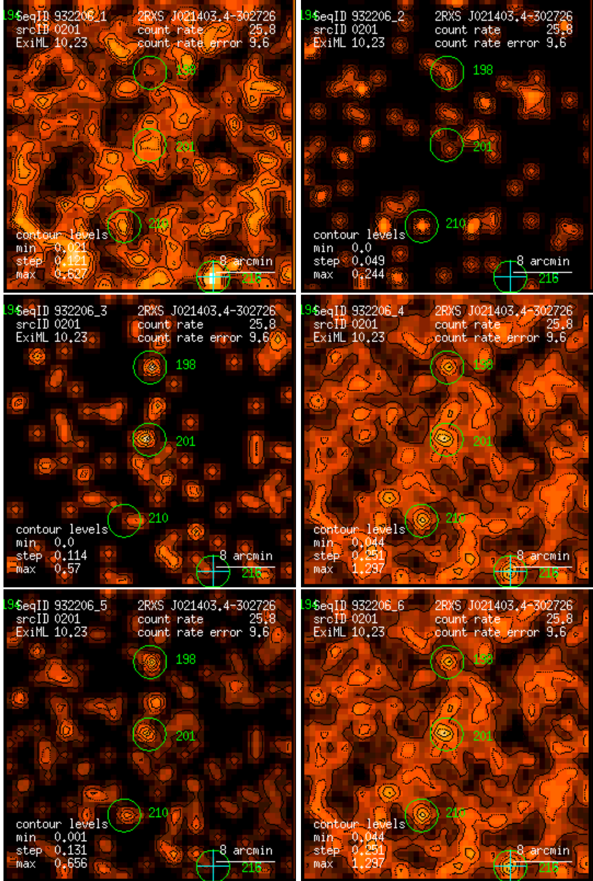
Figure 201: RASS 932206: detection 0201: band rate images, Gaussian filter: (1) PSPC channels 11 – 41, (2) 52 – 90, (3) 91 – 201, (4) 11 – 235, (5) 52 – 201, (6) 11 – 201. Broad band rates in counts/ks. Band rate contour levels in counts/ks/arcmin 2 .
