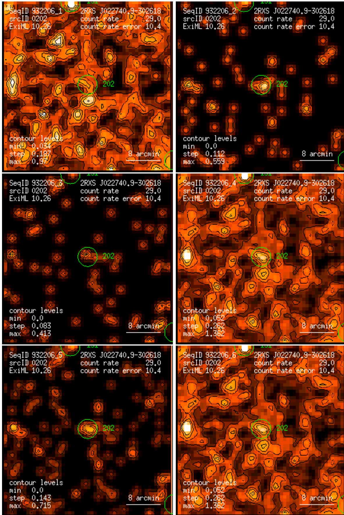
Figure 202: RASS 932206: detection 0202: band rate images, Gaussian filter: (1) PSPC channels 11 – 41, (2) 52 – 90, (3) 91 – 201, (4) 11 – 235, (5) 52 – 201, (6) 11 – 201. Broad band rates in counts/ks. Band rate contour levels in counts/ks/arcmin 2 .
