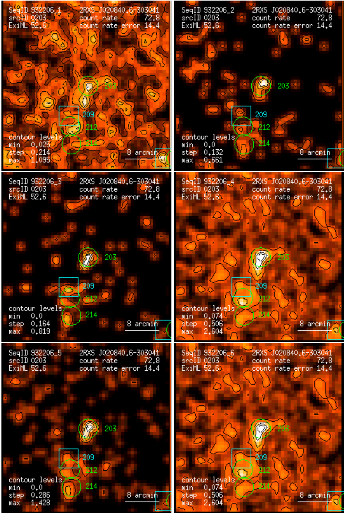
Figure 203: RASS 932206: detection 0203: band rate images, Gaussian filter: (1) PSPC channels 11 – 41, (2) 52 – 90, (3) 91 – 201, (4) 11 – 235, (5) 52 – 201, (6) 11 – 201. Broad band rates in counts/ks. Band rate contour levels in counts/ks/arcmin 2 .
