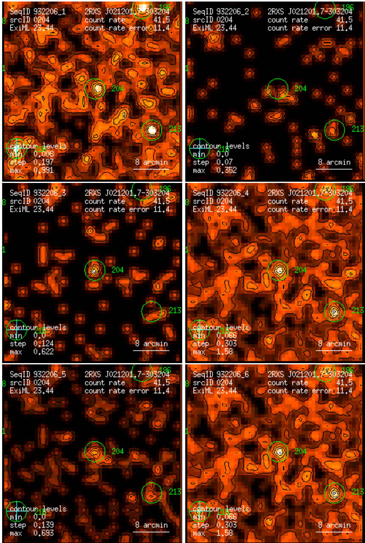
Figure 204: RASS 932206: detection 0204: band rate images, Gaussian filter: (1) PSPC channels 11 – 41, (2) 52 – 90, (3) 91 – 201, (4) 11 – 235, (5) 52 – 201, (6) 11 – 201. Broad band rates in counts/ks. Band rate contour levels in counts/ks/arcmin 2 .
