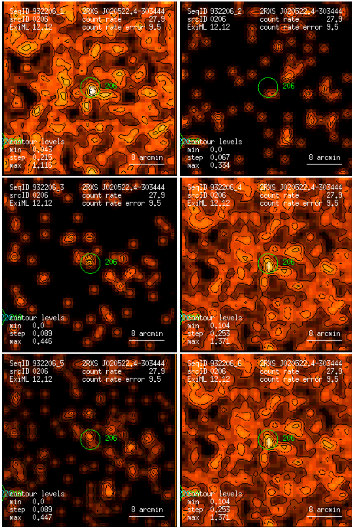
Figure 206: RASS 932206: detection 0206: band rate images, Gaussian filter: (1) PSPC channels 11 – 41, (2) 52 – 90, (3) 91 – 201, (4) 11 – 235, (5) 52 – 201, (6) 11 – 201. Broad band rates in counts/ks. Band rate contour levels in counts/ks/arcmin 2 .
