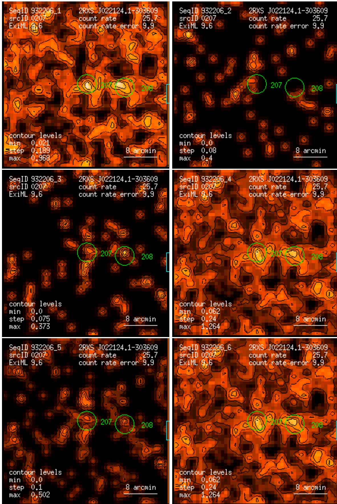
Figure 207: RASS 932206: detection 0207: band rate images, Gaussian filter: (1) PSPC channels 11 – 41, (2) 52 – 90, (3) 91 – 201, (4) 11 – 235, (5) 52 – 201, (6) 11 – 201. Broad band rates in counts/ks. Band rate contour levels in counts/ks/arcmin 2 .
