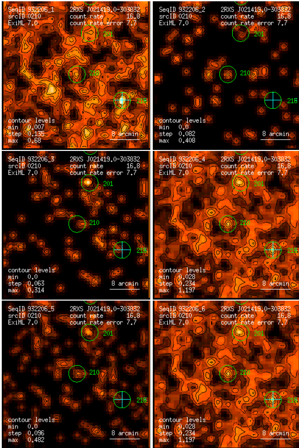
Figure 210: RASS 932206: detection 0210: band rate images, Gaussian filter: (1) PSPC channels 11 – 41, (2) 52 – 90, (3) 91 – 201, (4) 11 – 235, (5) 52 – 201, (6) 11 – 201. Broad band rates in counts/ks. Band rate contour levels in counts/ks/arcmin 2 .
