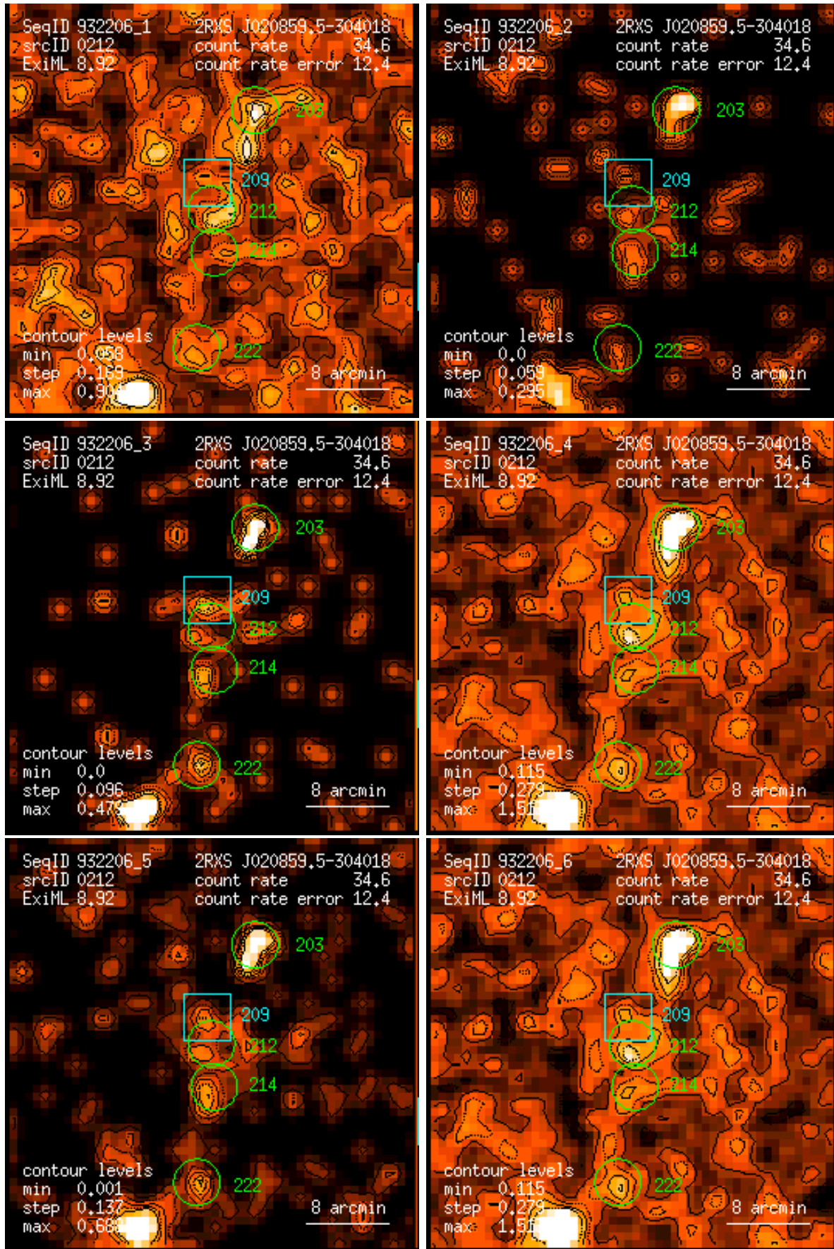
Figure 212: RASS 932206: detection 0212: band rate images, Gaussian filter: (1) PSPC channels 11 – 41, (2) 52 – 90, (3) 91 – 201, (4) 11 – 235, (5) 52 – 201, (6) 11 – 201. Broad band rates in counts/ks. Band rate contour levels in counts/ks/arcmin 2 .
