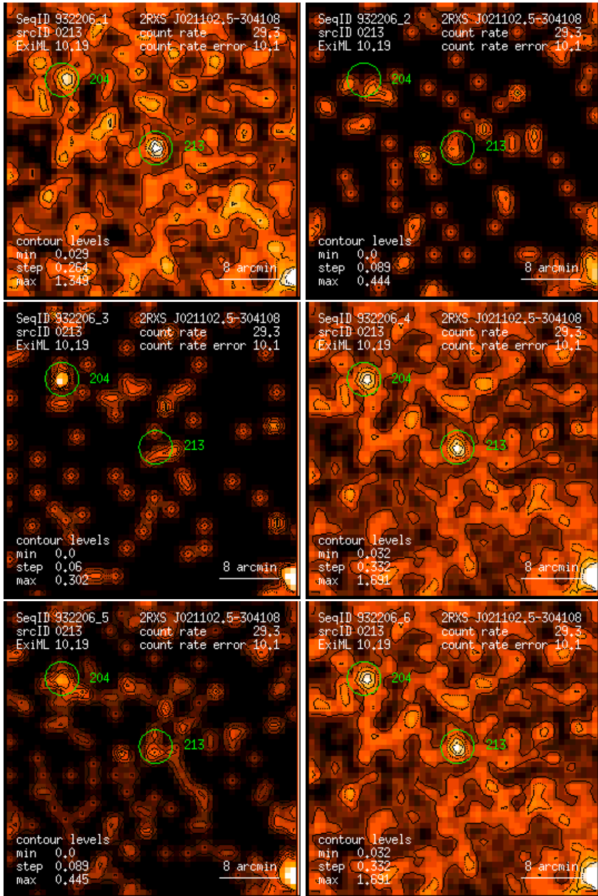
Figure 213: RASS 932206: detection 0213: band rate images, Gaussian filter: (1) PSPC channels 11 – 41, (2) 52 – 90, (3) 91 – 201, (4) 11 – 235, (5) 52 – 201, (6) 11 – 201. Broad band rates in counts/ks. Band rate contour levels in counts/ks/arcmin 2 .
