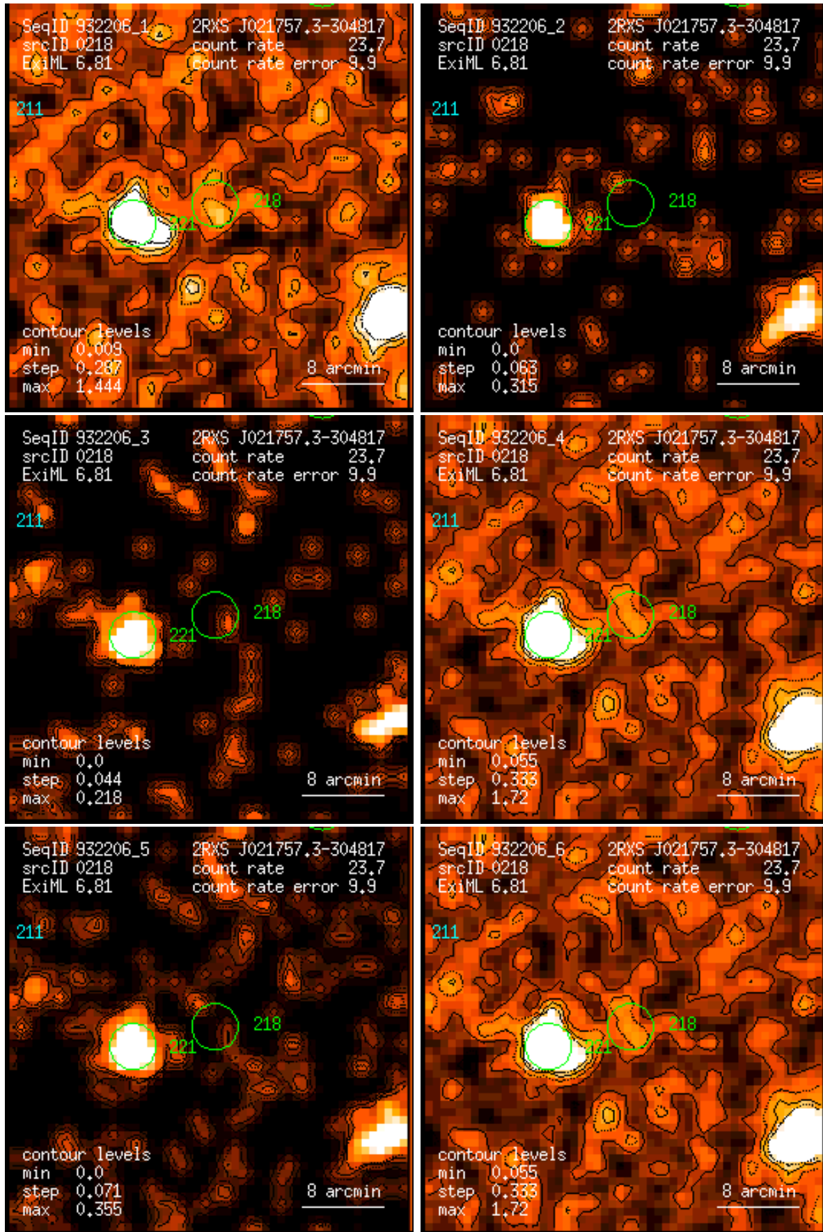
Figure 218: RASS 932206: detection 0218: band rate images, Gaussian filter: (1) PSPC channels 11 – 41, (2) 52 – 90, (3) 91 – 201, (4) 11 – 235, (5) 52 – 201, (6) 11 – 201. Broad band rates in counts/ks. Band rate contour levels in counts/ks/arcmin 2 .
