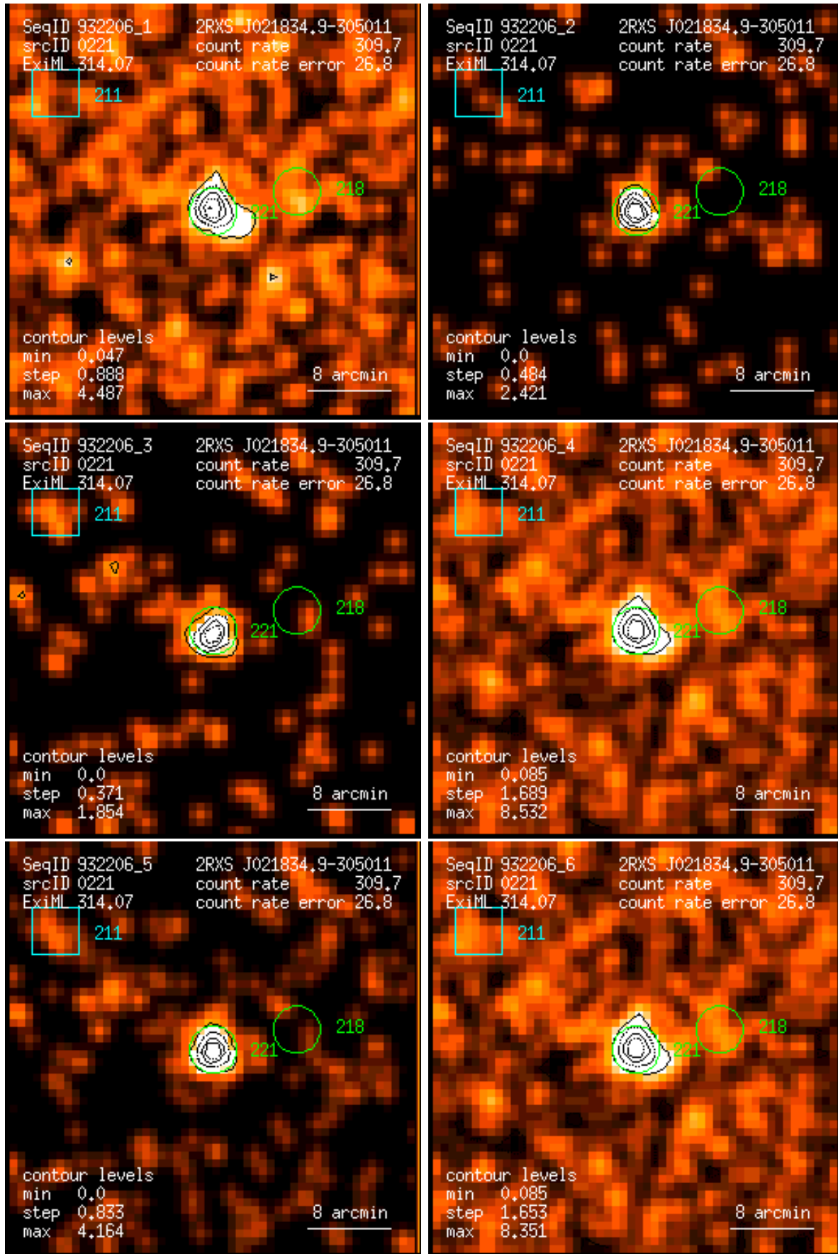
Figure 221: RASS 932206: detection 0221: band rate images, Gaussian filter: (1) PSPC channels 11 – 41, (2) 52 – 90, (3) 91 – 201, (4) 11 – 235, (5) 52 – 201, (6) 11 – 201. Broad band rates in counts/ks. Band rate contour levels in counts/ks/arcmin 2 .
