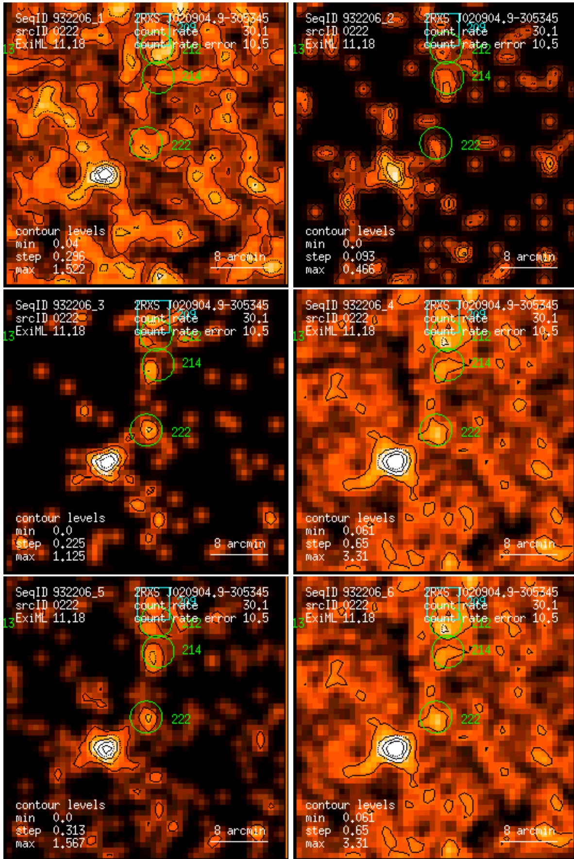
Figure 222: RASS 932206: detection 0222: band rate images, Gaussian filter: (1) PSPC channels 11 – 41, (2) 52 – 90, (3) 91 – 201, (4) 11 – 235, (5) 52 – 201, (6) 11 – 201. Broad band rates in counts/ks. Band rate contour levels in counts/ks/arcmin 2 .
