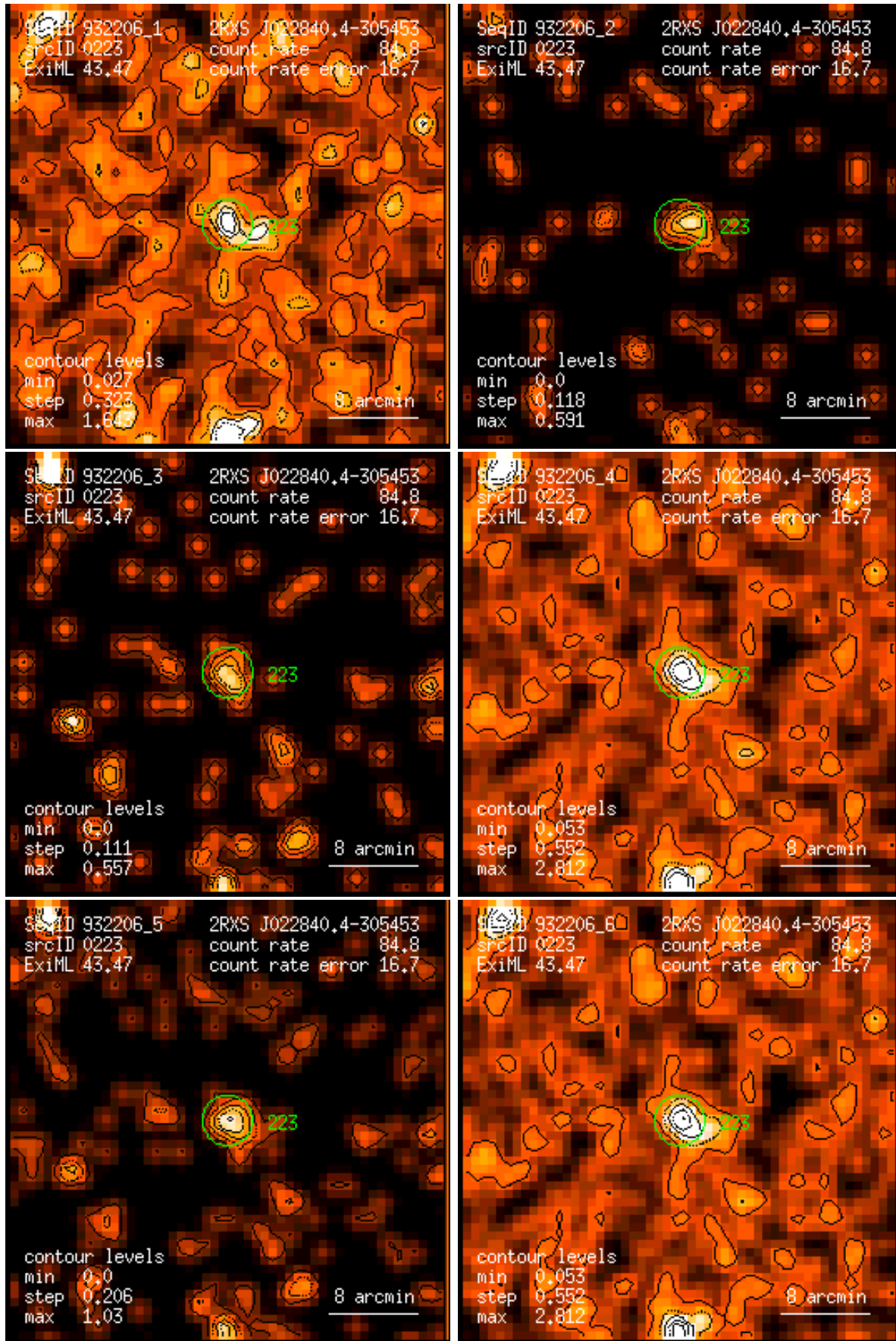
Figure 223: RASS 932206: detection 0223: band rate images, Gaussian filter: (1) PSPC channels 11 – 41, (2) 52 – 90, (3) 91 – 201, (4) 11 – 235, (5) 52 – 201, (6) 11 – 201. Broad band rates in counts/ks. Band rate contour levels in counts/ks/arcmin 2 .
