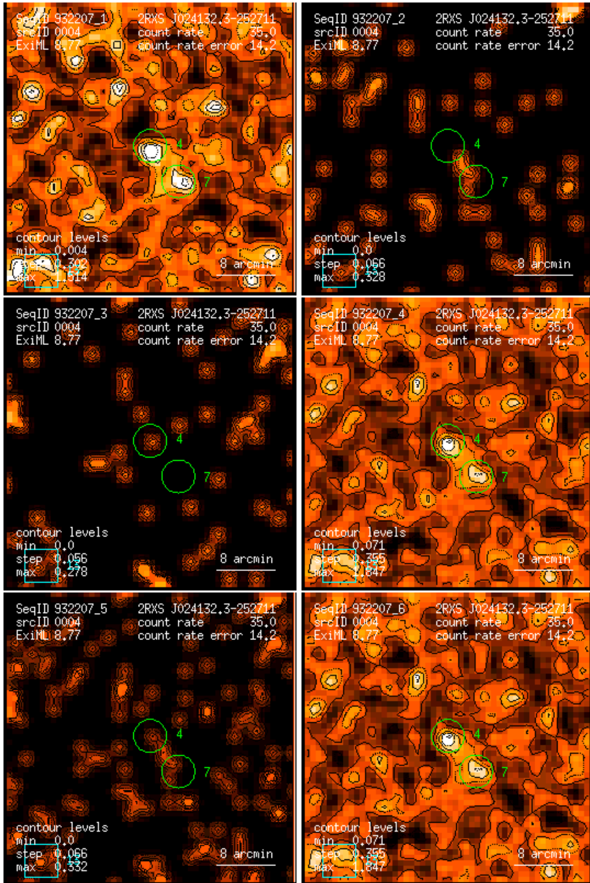
Figure 4: RASS 932207: detection 0004: band rate images, Gaussian filter: (1) PSPC channels 11 – 41, (2) 52 – 90, (3) 91 – 201, (4) 11 – 235, (5) 52 – 201, (6) 11 – 201. Broad band rates in counts/ks. Band rate contour levels in counts/ks/arcmin 2 .
