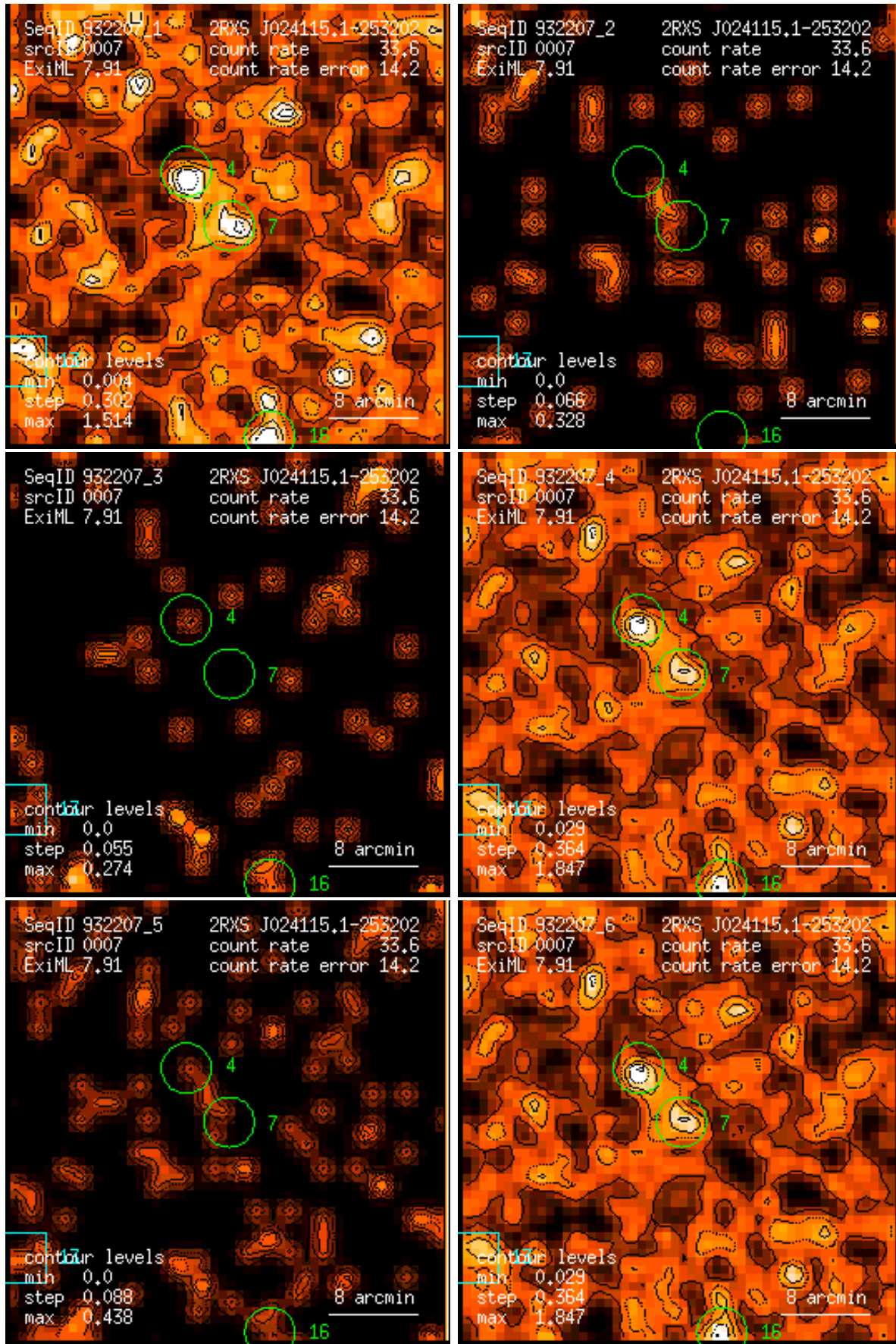
Figure 7: RASS 932207: detection 0007: band rate images, Gaussian filter: (1) PSPC channels 11 – 41, (2) 52 – 90, (3) 91 – 201, (4) 11 – 235, (5) 52 – 201, (6) 11 – 201. Broad band rates in counts/ks. Band rate contour levels in counts/ks/arcmin 2 .
