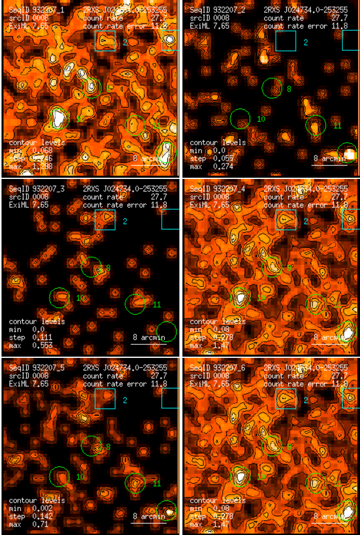
Figure 8: RASS 932207: detection 0008: band rate images, Gaussian filter: (1) PSPC channels 11 – 41, (2) 52 – 90, (3) 91 – 201, (4) 11 – 235, (5) 52 – 201, (6) 11 – 201. Broad band rates in counts/ks. Band rate contour levels in counts/ks/arcmin 2 .
