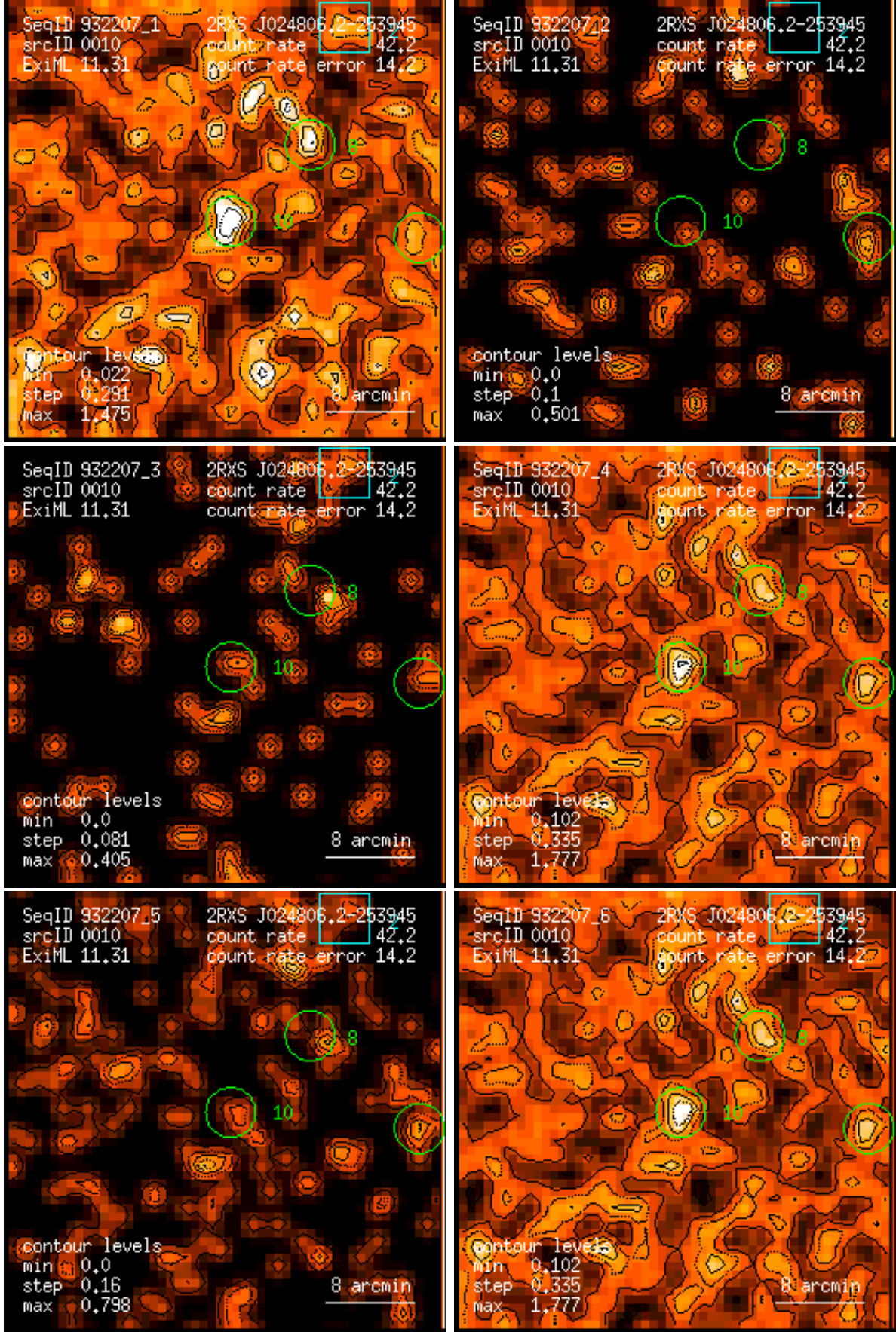
Figure 10: RASS 932207: detection 0010: band rate images, Gaussian filter: (1) PSPC channels 11 – 41, (2) 52 – 90, (3) 91 – 201, (4) 11 – 235, (5) 52 – 201, (6) 11 – 201. Broad band rates in counts/ks. Band rate contour levels in counts/ks/arcmin 2 .
