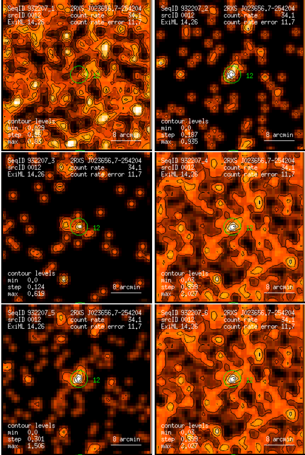
Figure 12: RASS 932207: detection 0012: band rate images, Gaussian filter: (1) PSPC channels 11 – 41, (2) 52 – 90, (3) 91 – 201, (4) 11 – 235, (5) 52 – 201, (6) 11 – 201. Broad band rates in counts/ks. Band rate contour levels in counts/ks/arcmin 2 .
