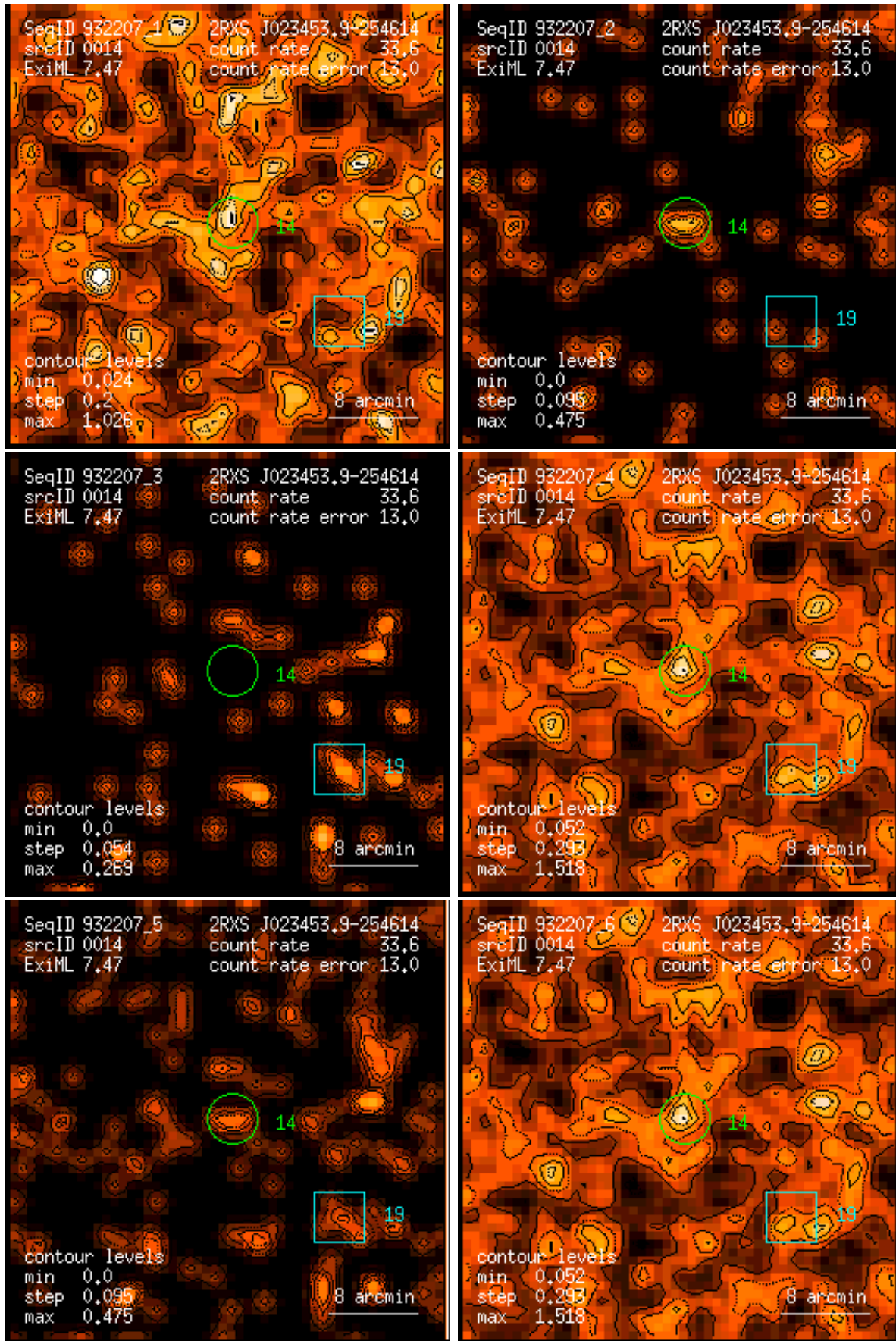
Figure 14: RASS 932207: detection 0014: band rate images, Gaussian filter: (1) PSPC channels 11 – 41, (2) 52 – 90, (3) 91 – 201, (4) 11 – 235, (5) 52 – 201, (6) 11 – 201. Broad band rates in counts/ks. Band rate contour levels in counts/ks/arcmin 2 .
