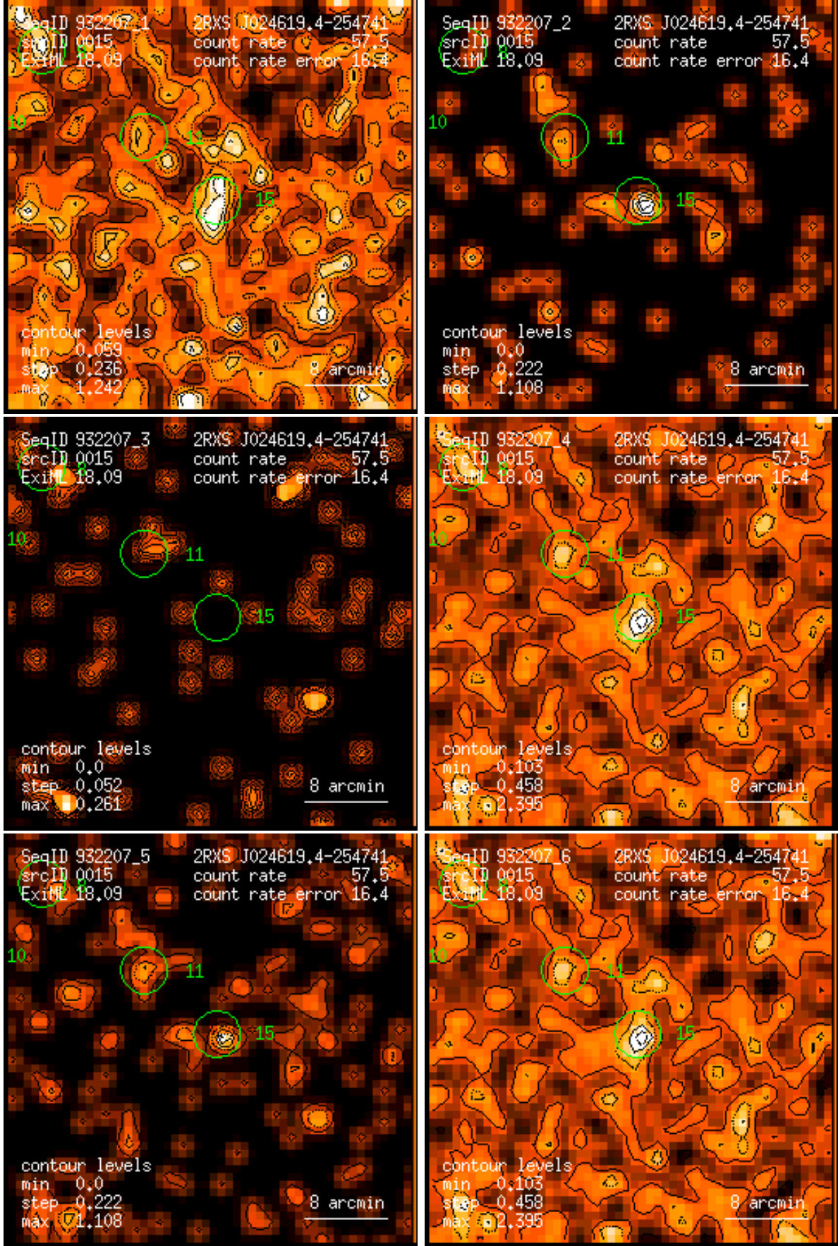
Figure 15: RASS 932207: detection 0015: band rate images, Gaussian filter: (1) PSPC channels 11 – 41, (2) 52 – 90, (3) 91 – 201, (4) 11 – 235, (5) 52 – 201, (6) 11 – 201. Broad band rates in counts/ks. Band rate contour levels in counts/ks/arcmin 2 .
