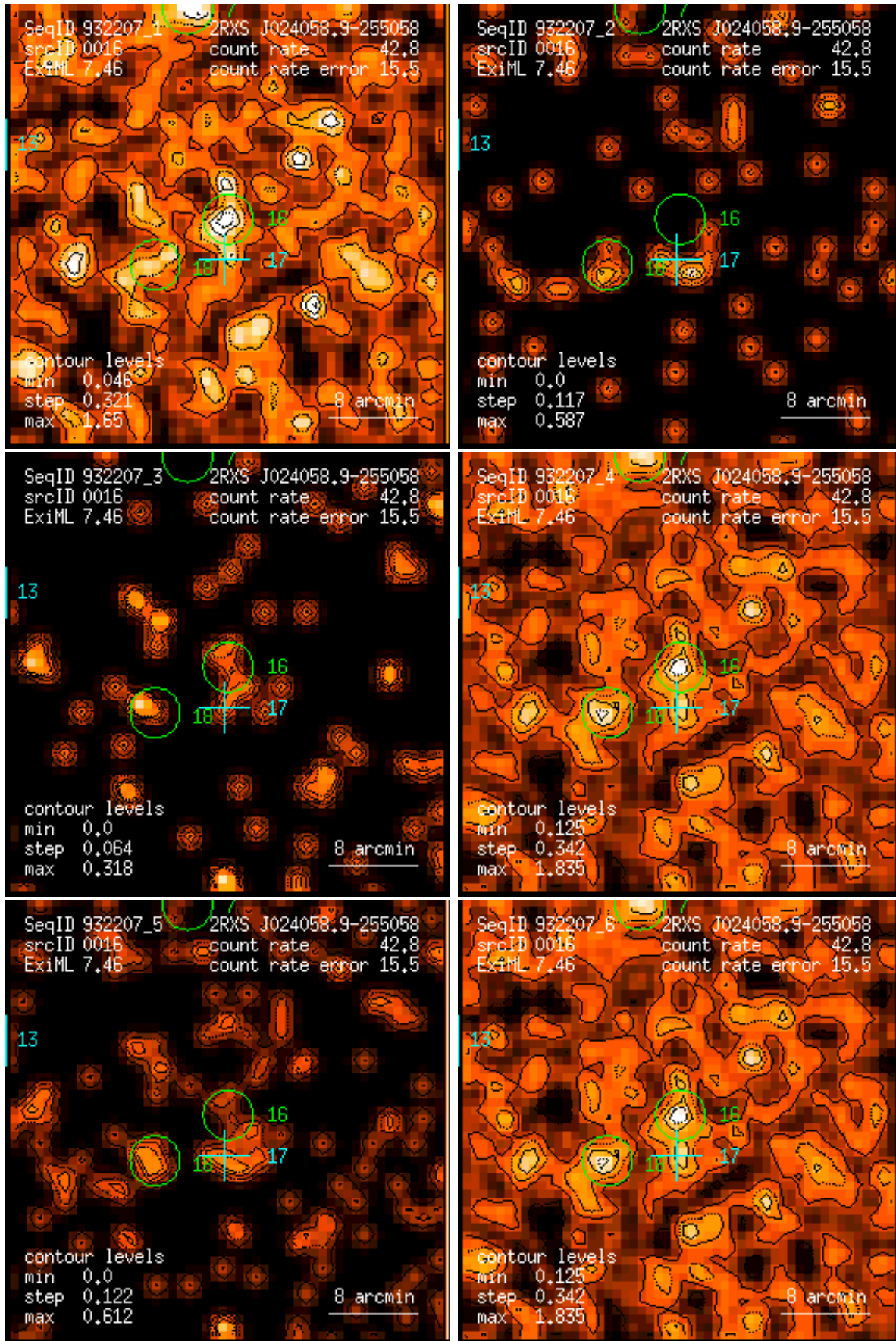
Figure 16: RASS 932207: detection 0016: band rate images, Gaussian filter: (1) PSPC channels 11 – 41, (2) 52 – 90, (3) 91 – 201, (4) 11 – 235, (5) 52 – 201, (6) 11 – 201. Broad band rates in counts/ks. Band rate contour levels in counts/ks/arcmin 2 .
