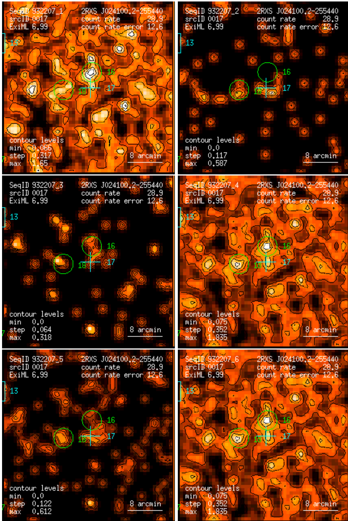
Figure 17: RASS 932207: detection 0017: band rate images, Gaussian filter: (1) PSPC channels 11 – 41, (2) 52 – 90, (3) 91 – 201, (4) 11 – 235, (5) 52 – 201, (6) 11 – 201. Broad band rates in counts/ks. Band rate contour levels in counts/ks/arcmin 2 .
